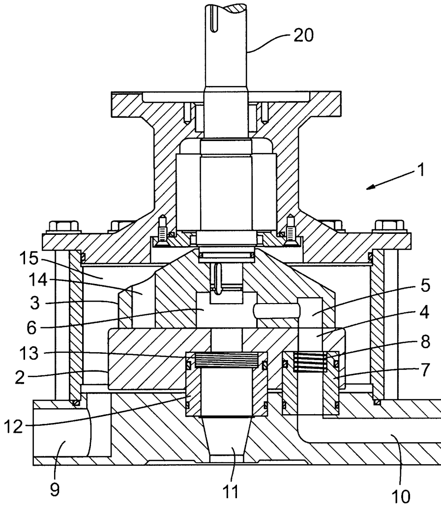
FIG. 1 Prior Art
