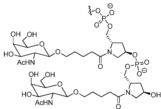
Formula XXXI;
