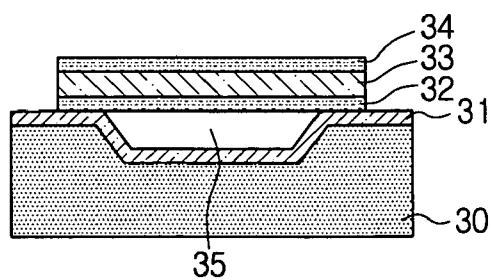
FIG. 1C (PRIOR ART)
