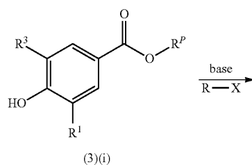
Scheme 3
