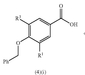
Scheme 4
