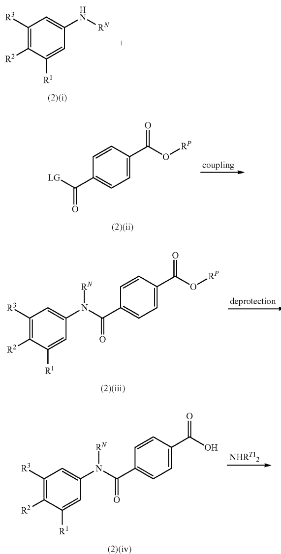
Scheme 2
