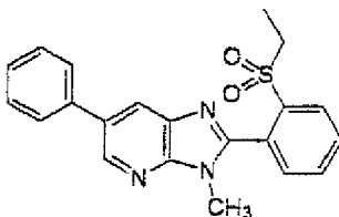
Present Compound 57
