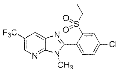
Present Compound 135
