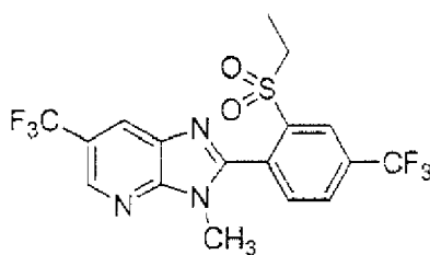
Present Compound 176
