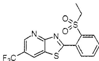
Present Compound 329
