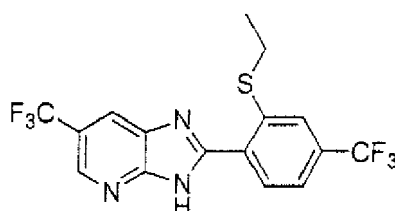
Present Compound 344
