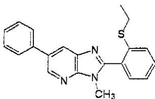
Present Compound 56
