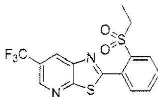
Present Compound 185
