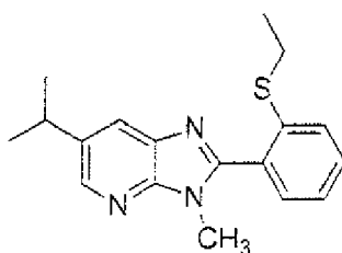
Present Compound 147
