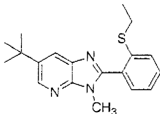
Present Compound 150
