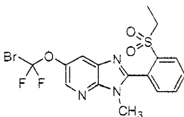
Present Compound 270
