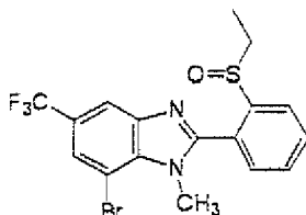
Present Compound 75
