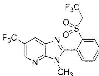
Present Compound 187
