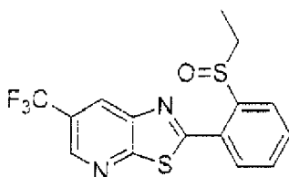
Present Compound 184
