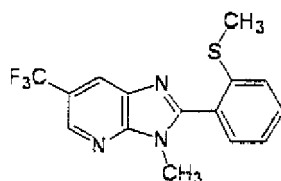
Present Compound 1
