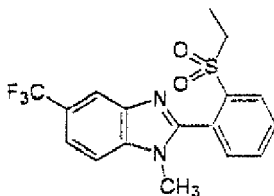
Present Compound 70
