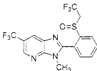
Present Compound 187
