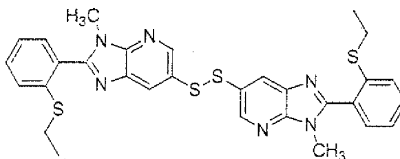
Compound (145A)
