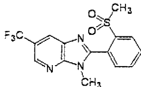
Present Compound 3
