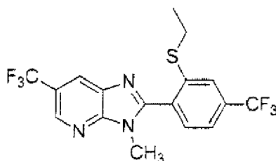
Present Compound 174
