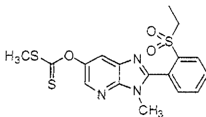
Compound 270A
