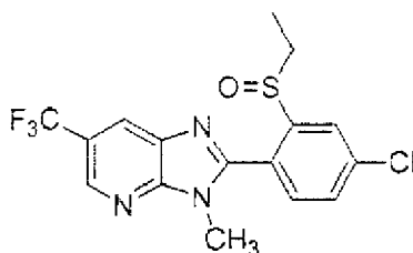
Present Compound 134
