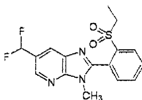
Present Compound 54
