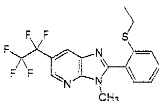
Present Compound 55
