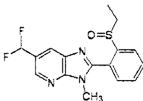
Present Compound 53
