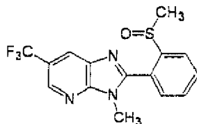
Present Compound 2
