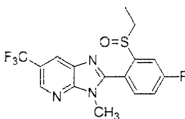
Present Compound 117
