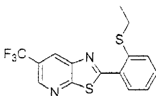
Present Compound 183
