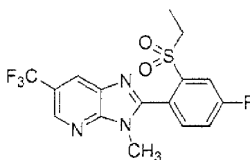
Present Compound 118
