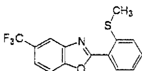
Present Compound 77
