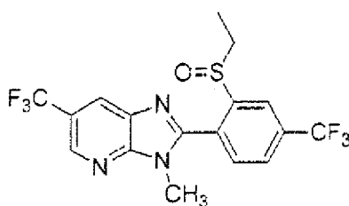
Present Compound 175
