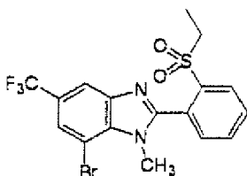
Present Compound 76
