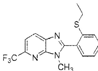
Present Compound 151
