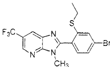
Present Compound 238
