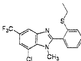
Present Compound 71
