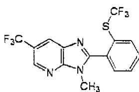
Present Compound 18
