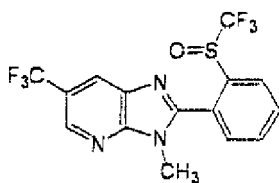
Present Compound 19
