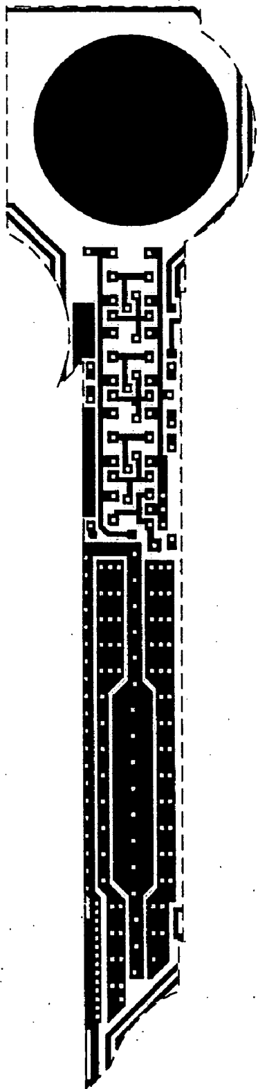
Metal 1 mask
