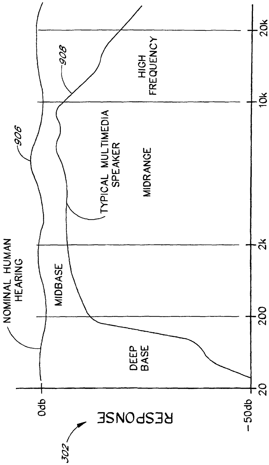
FREQUENCY 304 FIG. 9
