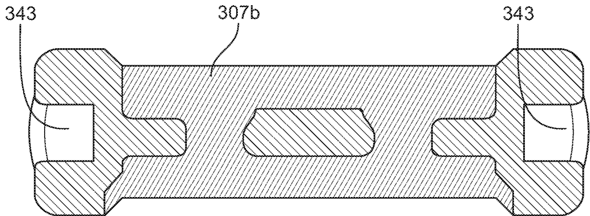
SECTION F-F
