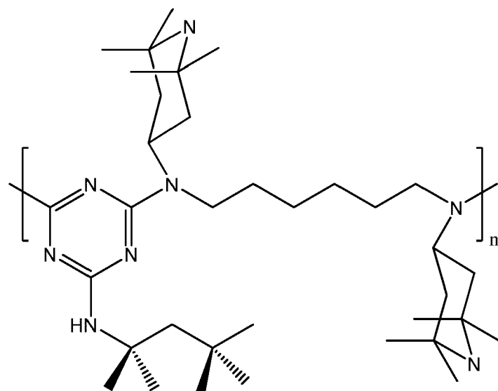
[Chemical Formula 2]
