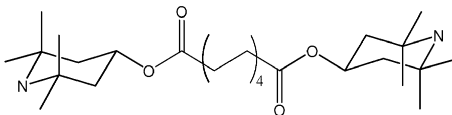
[Chemical Formula 2]
