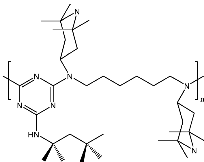
[Chemical Formula 2]
