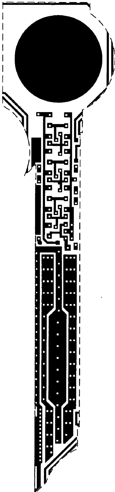
Metal 1 mask
