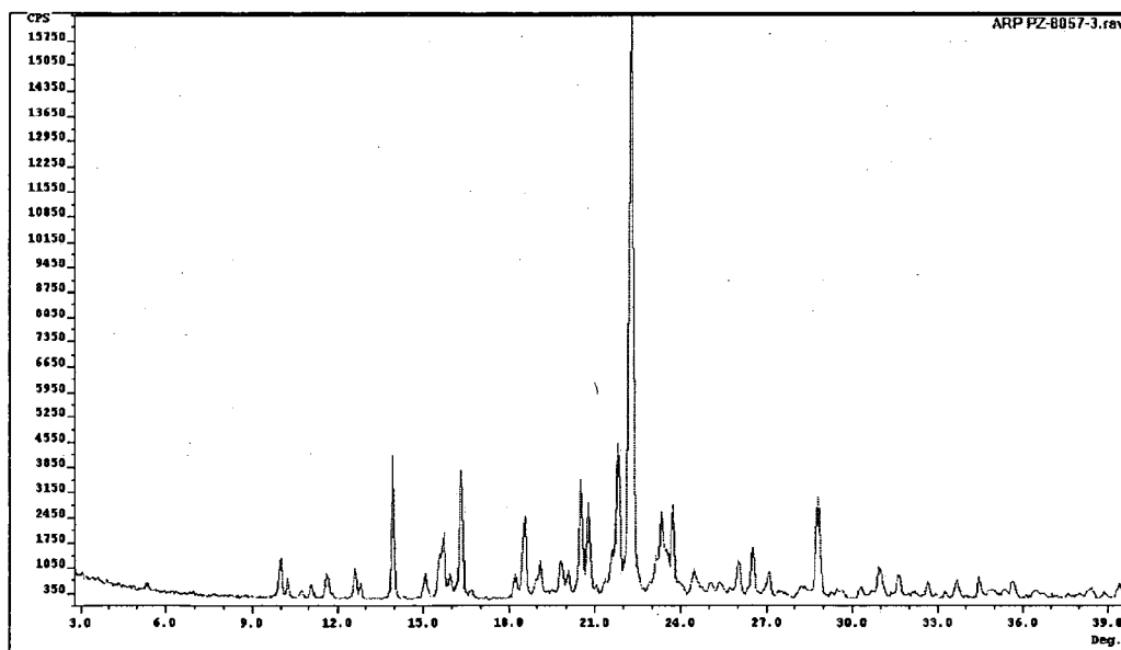
Figure 2. X-ray Diffractogram of Aripiprazole Type-II.
