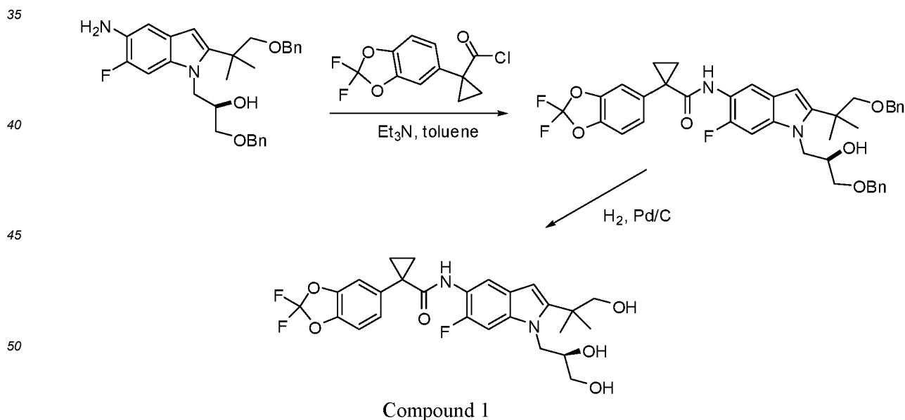
Scheme 4. Formation of Compound 1.
