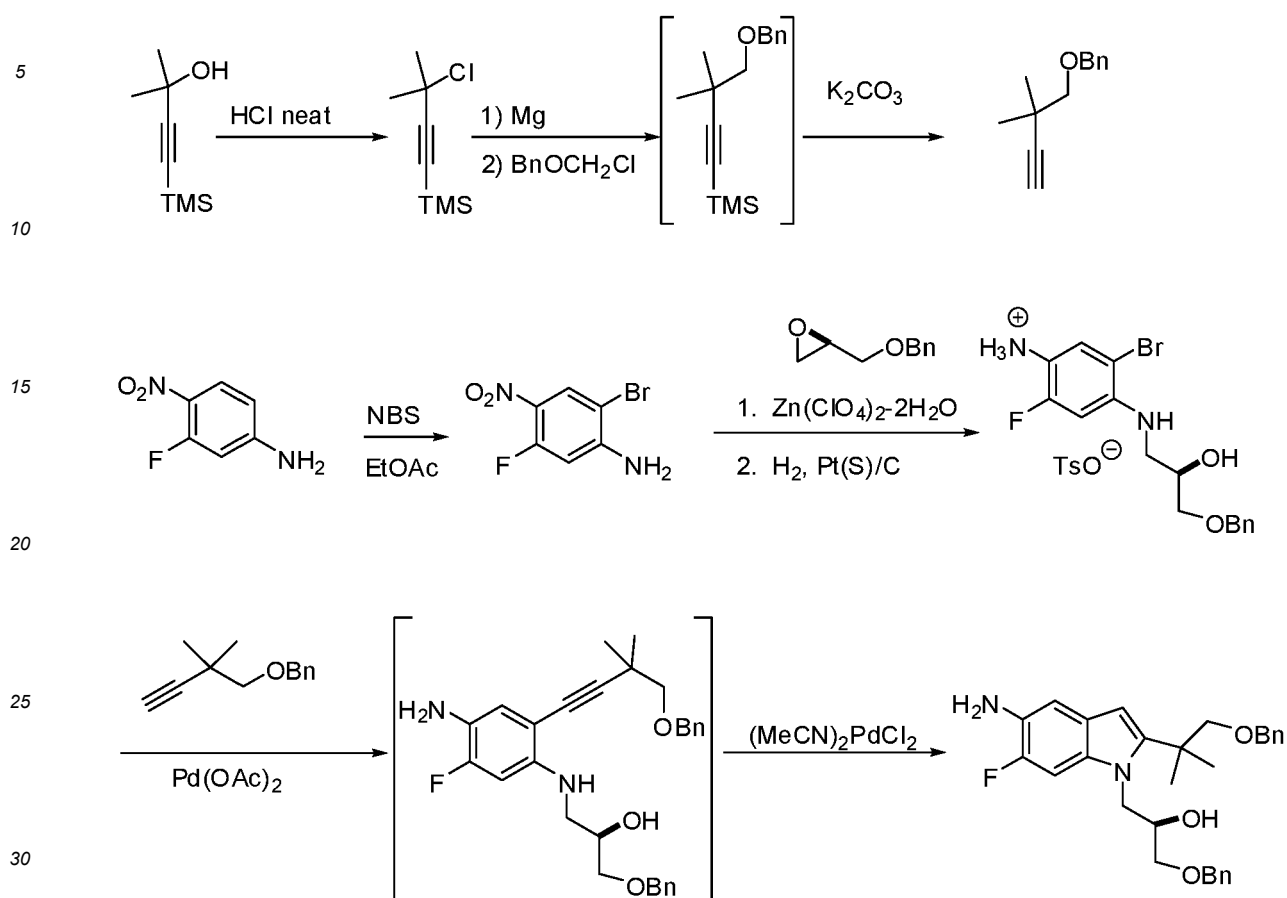
Scheme 4. Formation of Compound 1.
