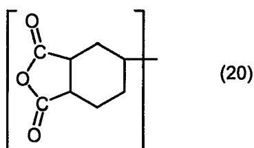
[Chemical Formula 7]
