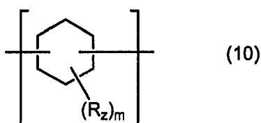
[Chemical Formula 6]
