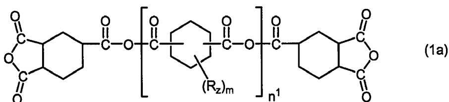
[Chemical Formula 8]
