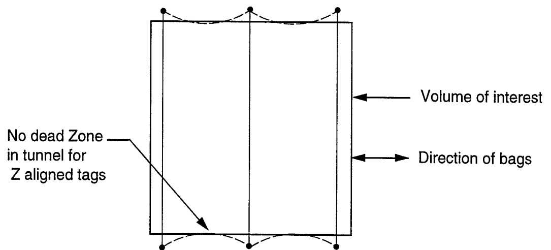
Fig 14. Three axis coils
