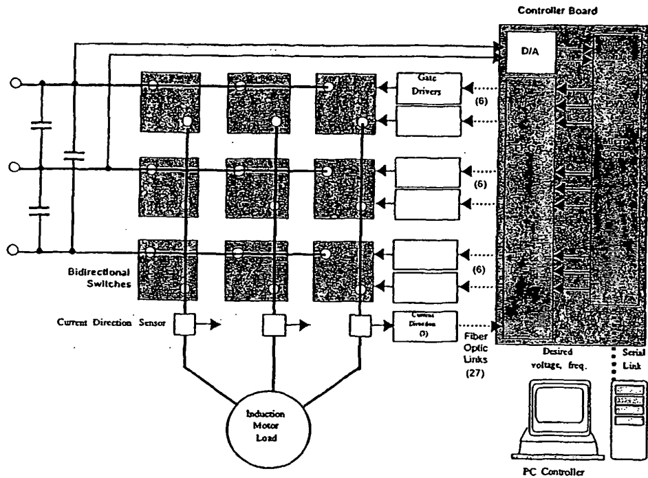
Figure 1: The Matrix Converter Circuit and Controller
