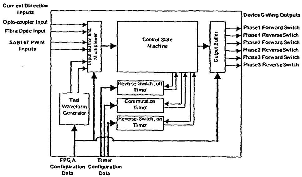
Figure 6 Schematic of the FPGA controller IC
