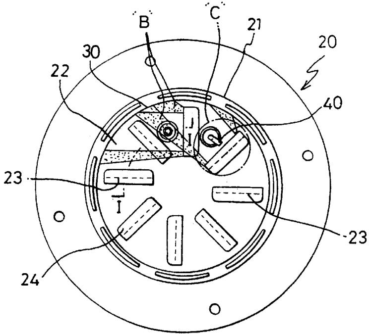
FIG. 4 Related Art
