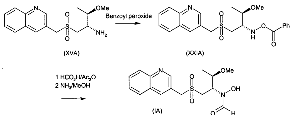
Scheme 5
