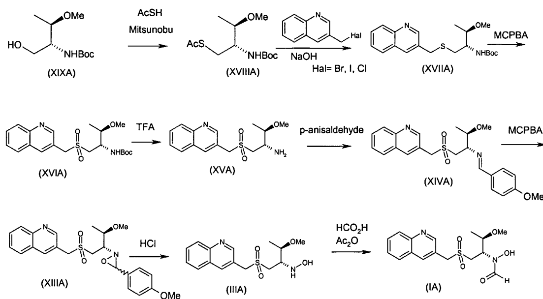
Scheme 3
