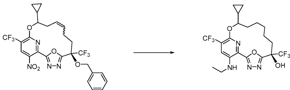
E/Z mixture
