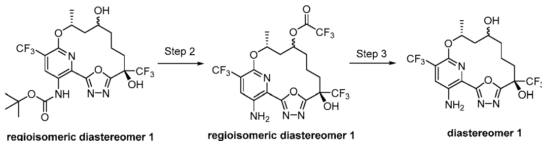
regioisomeric diastereomer 1
