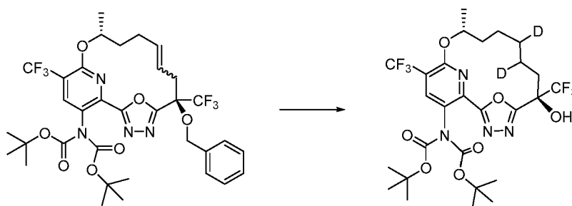
E/Z mixture
