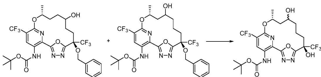
regioisomeric diastereomer 1
