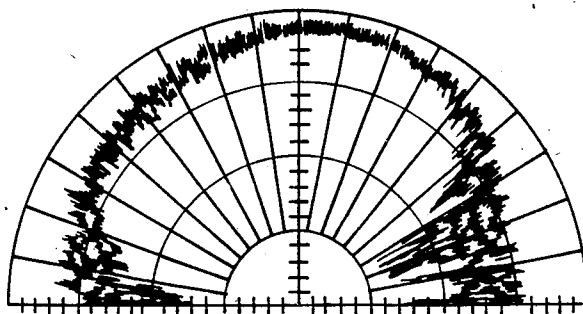
PLANAR/CONICAL/HELIX ANTENNA
