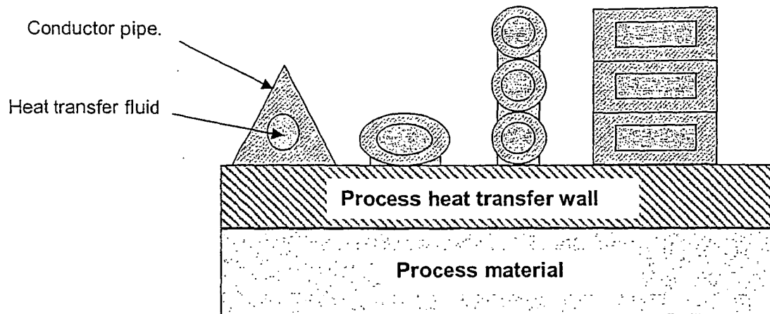
Examples of different conductor shapes and group arrangement
