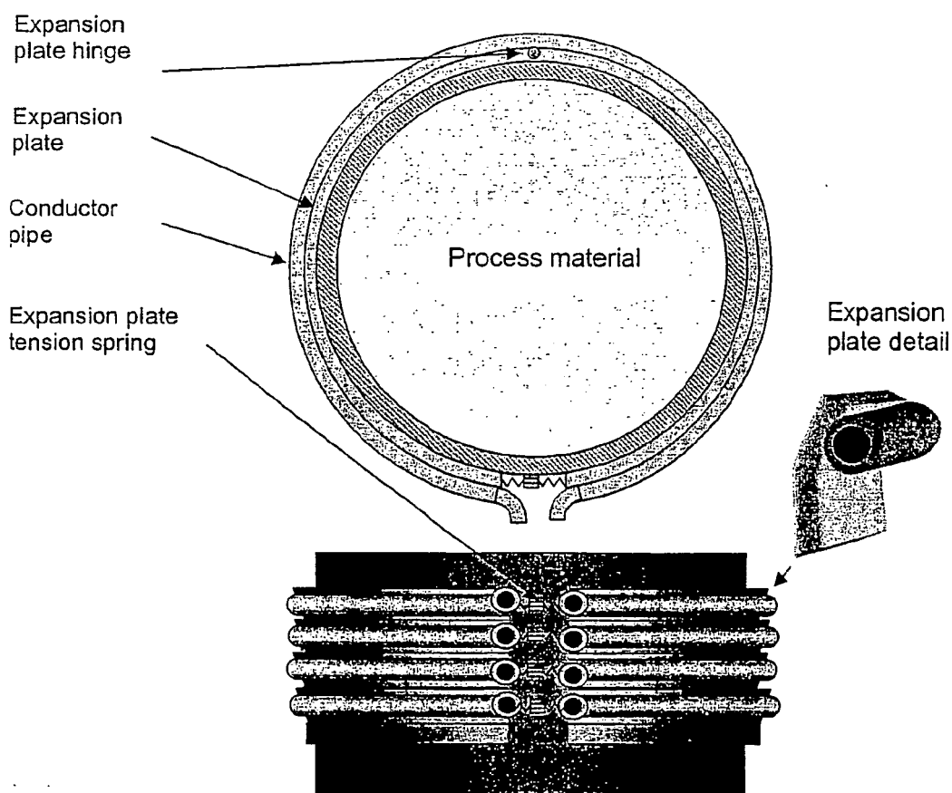
Expansion plates with an open profile
