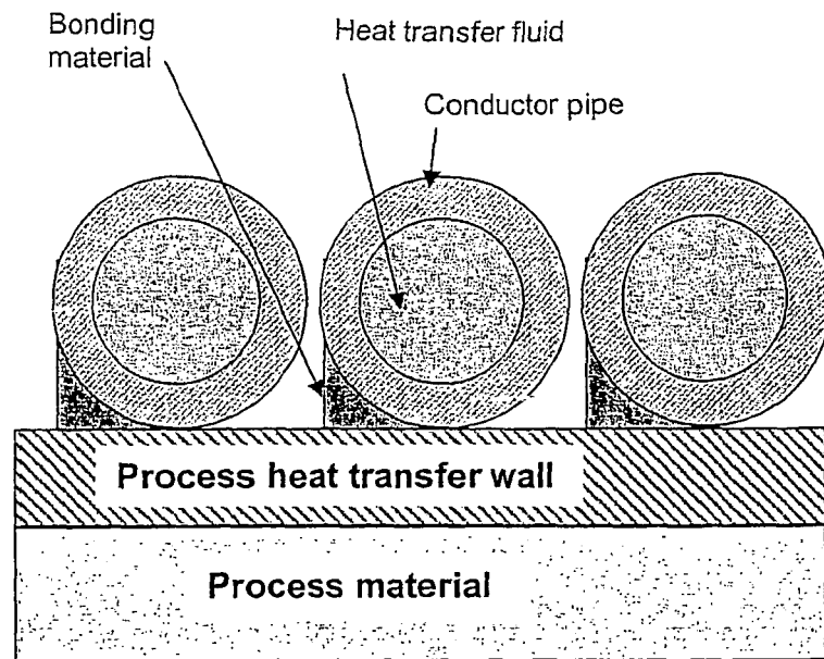
One-sided solder bonding
