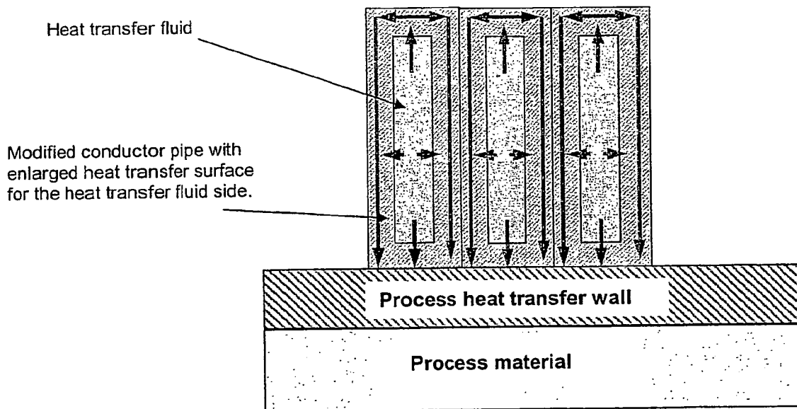
Section through oblong conductor pipes
