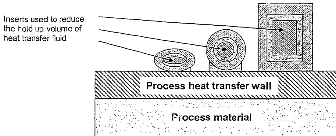
Examples of different inserts
