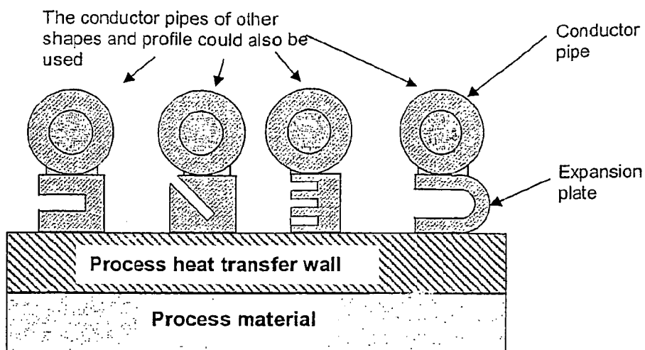
Examples of various expansion plate shapes
