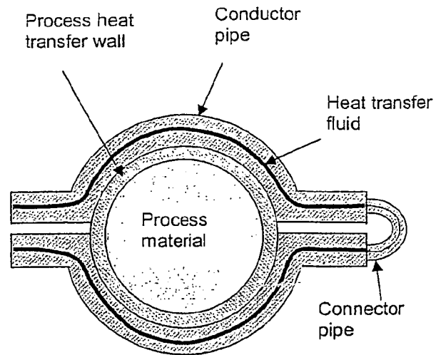
Two part mounted conductor pipe configuration
