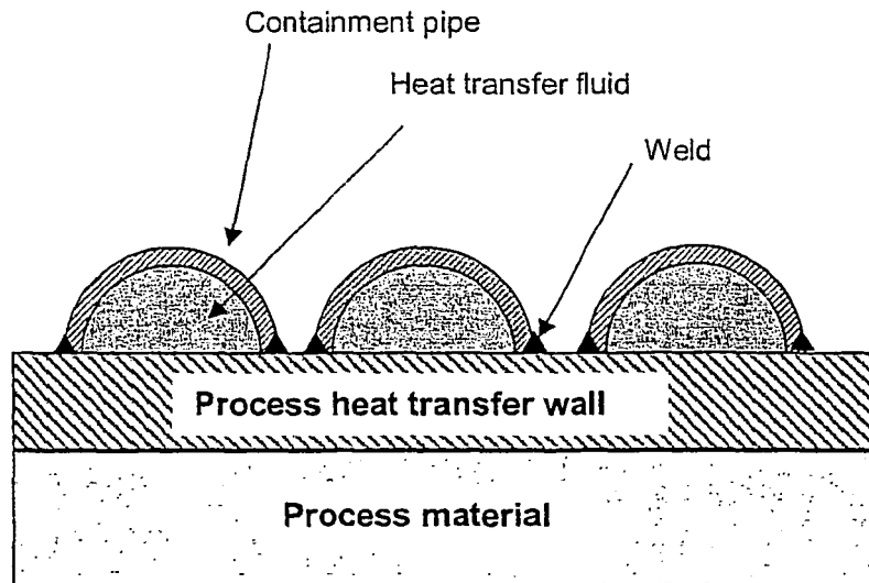
Conventional half coil welds
