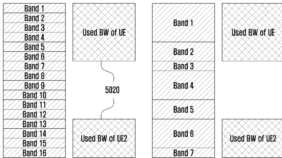
Case C: Static Partitioning with Fine Granularity
