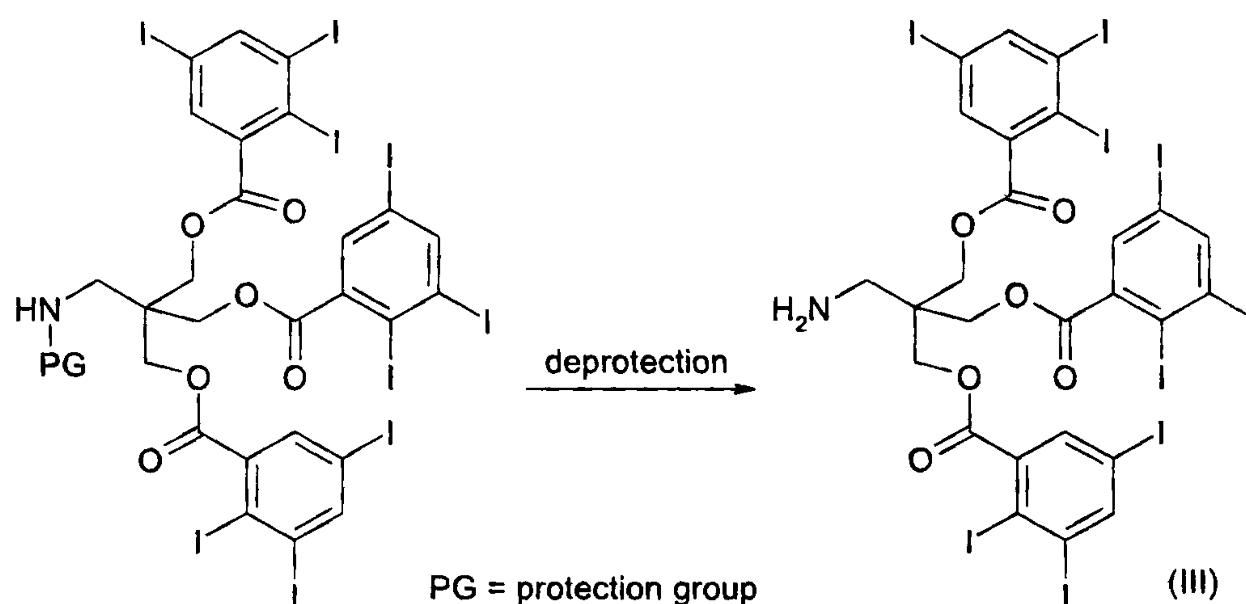
Scheme 2:
