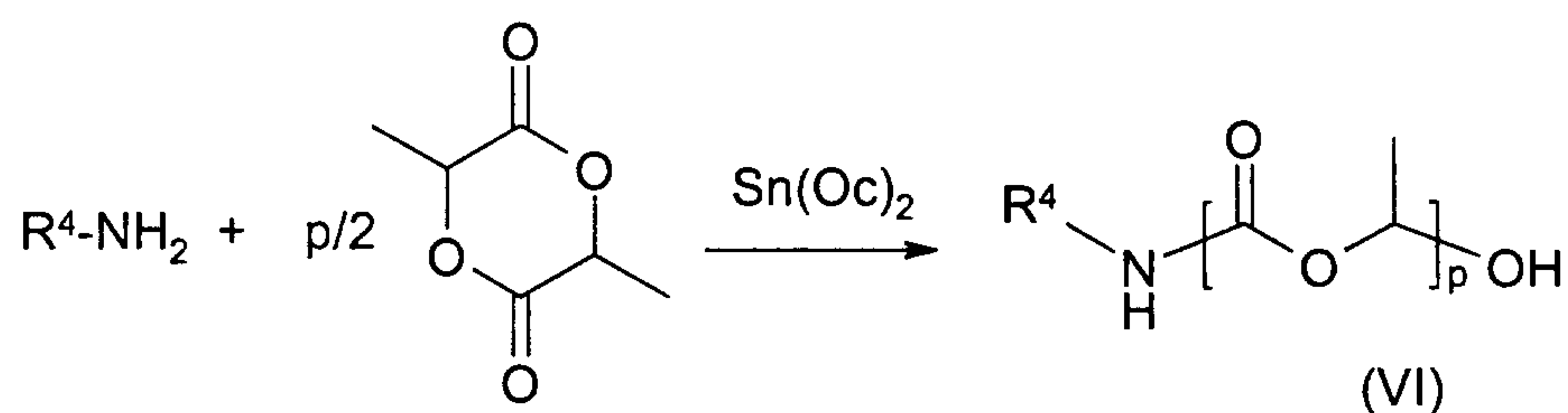
Scheme 4:
