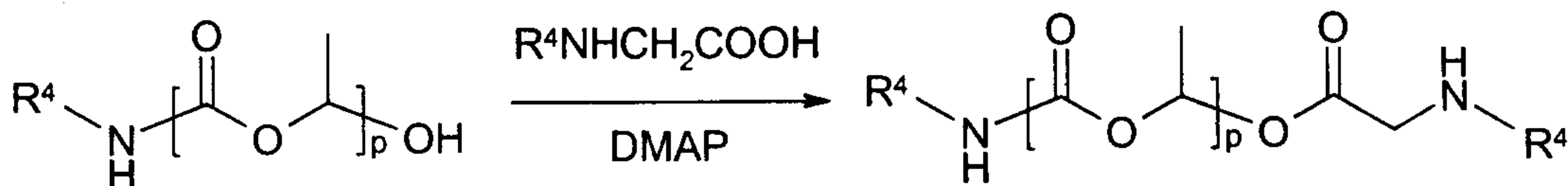
Scheme 6:
