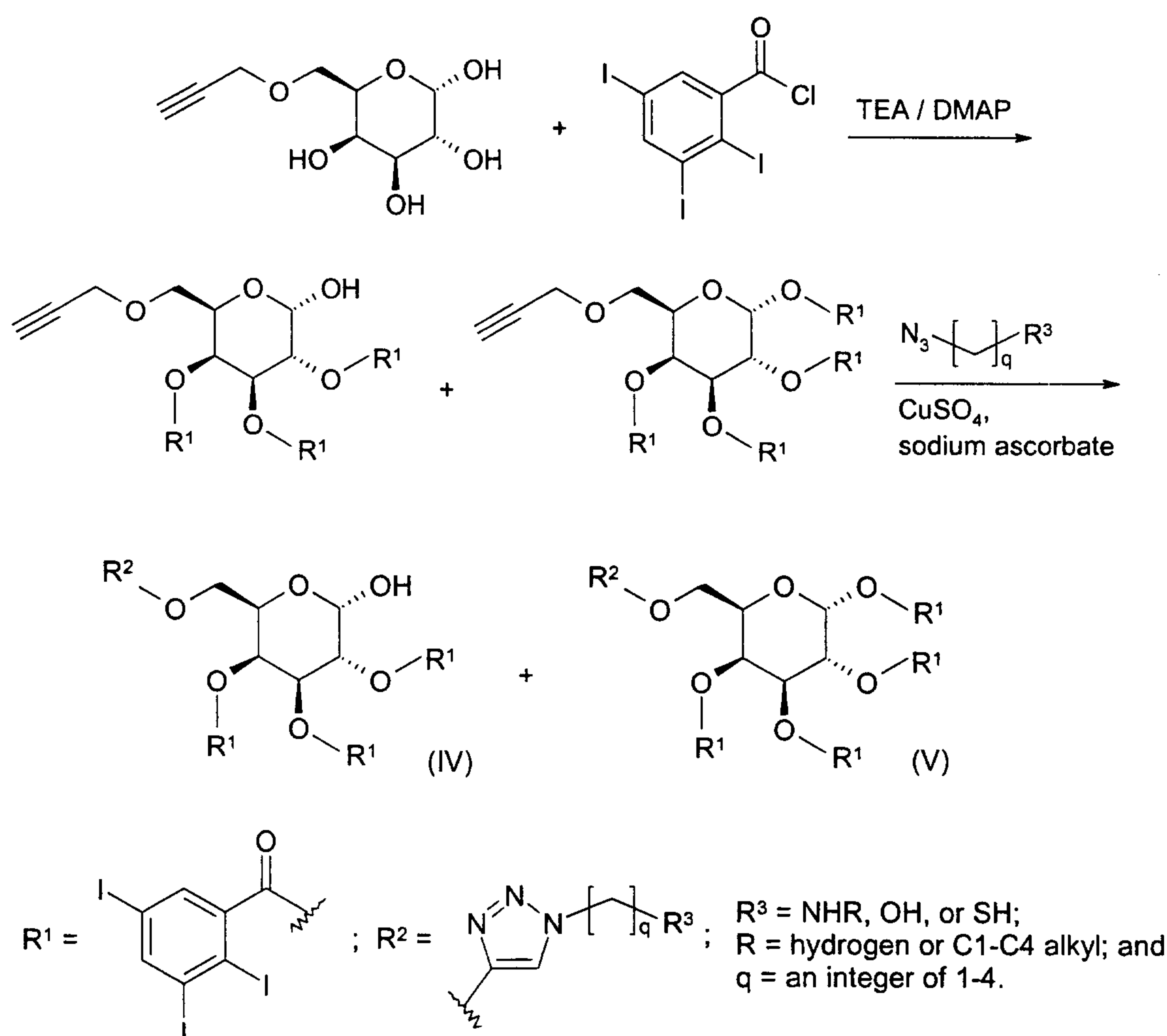
Scheme 3:
