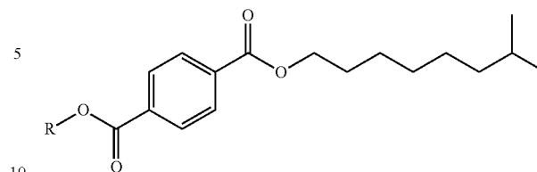
[Chemical Formula 1]
