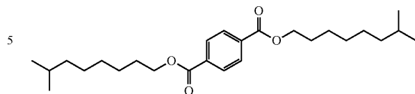
[Chemical Formula 3]
