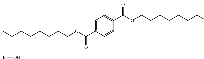
[Chemical Formula 4]
