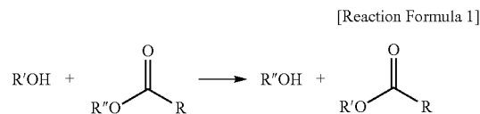
[Reaction Formula 1]
