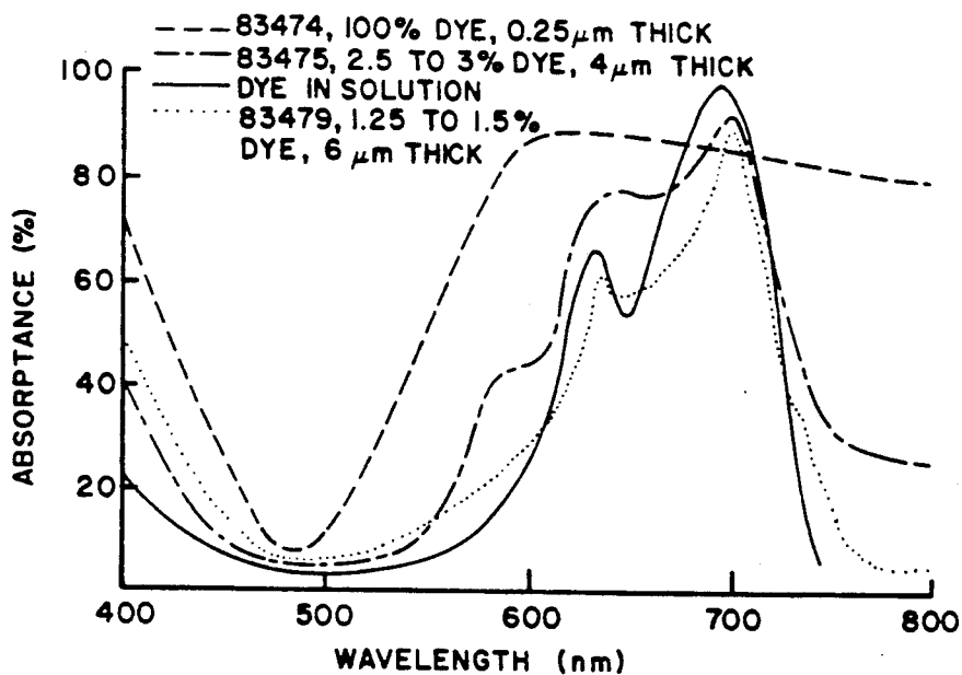
ABSORPTANCE SPECTRA OF THREE VOPc - POLYESTER FILMS
