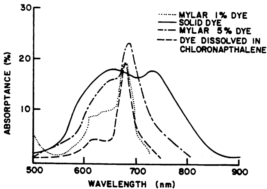
ABSORPTANCE SPECTRA OF THREE AlCl_2Pc - POLYESTER FILMS
