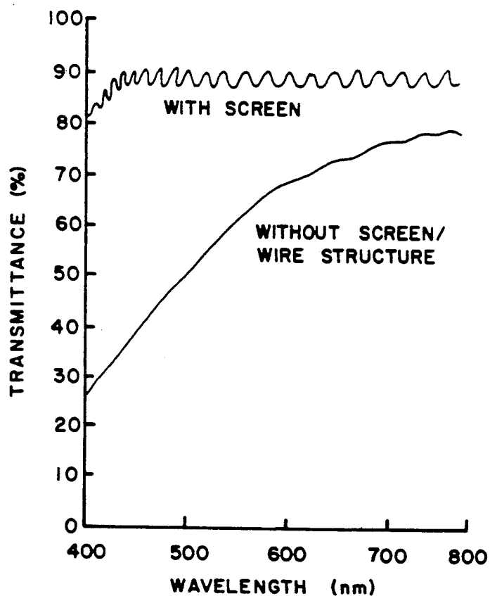
SPECTRAL TRANSMITTANCE OF POLYESTER FILMS
