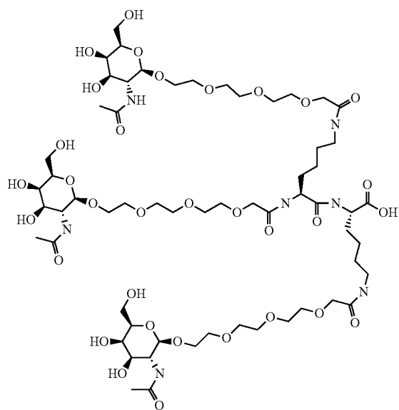
One embodiment of a Galactose cluster
