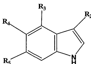
Formula IIa
