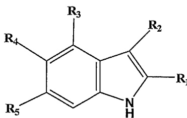
Formula IIa
