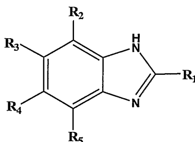
Formula III
