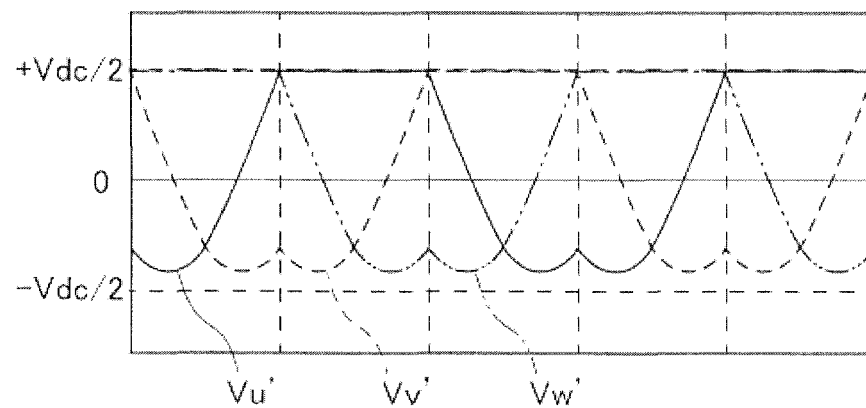
(c) SECOND PHASE VOLTAGE COMMAND VALUES S51
