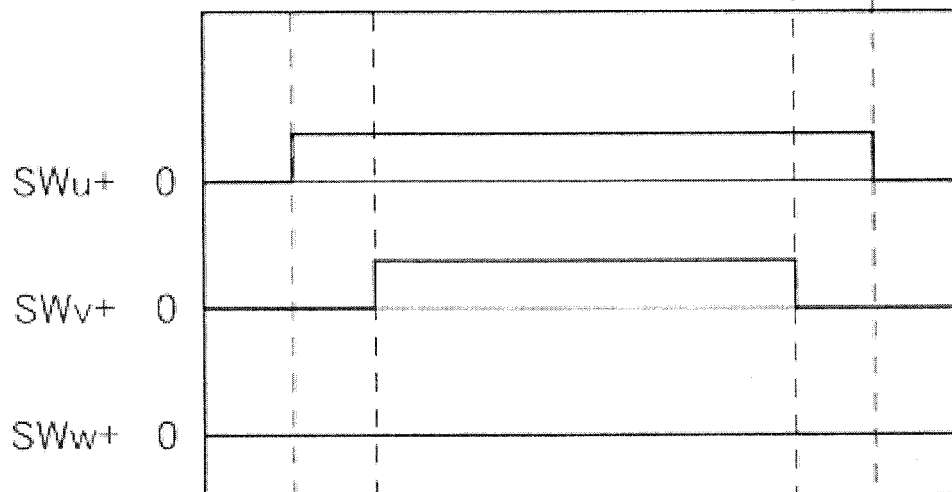
(b) SWITCHING SIGNALS S4
