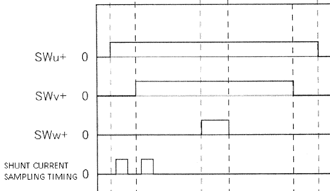
(b) SWITCHING SIGNALS S4
