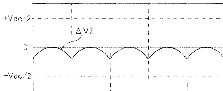
(c) SECOND PHASE VOLTAGE COMMAND VALUES S51
