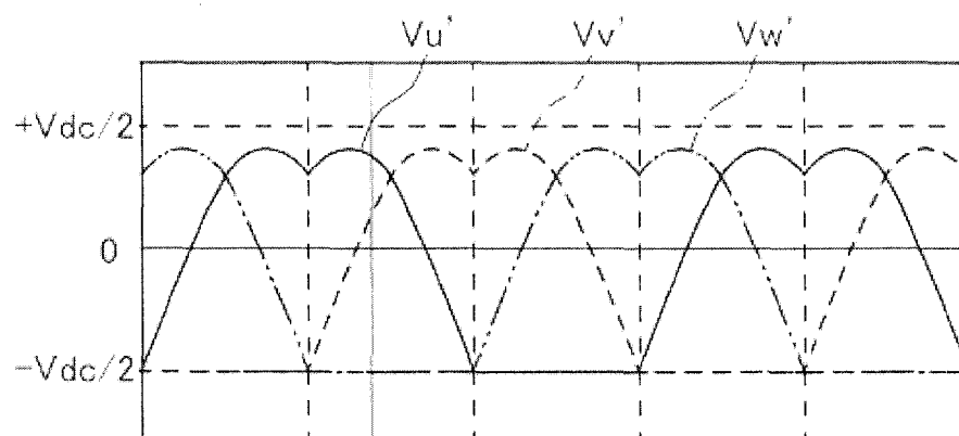
(c) SECOND PHASE VOLTAGE COMMAND VALUES S51
