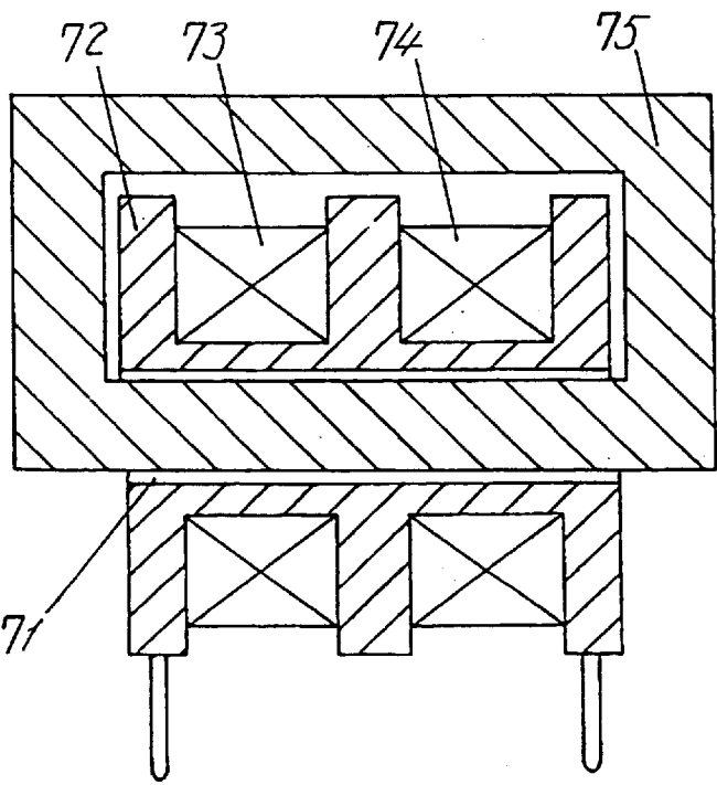
Fig. 30 PRIOR ART
