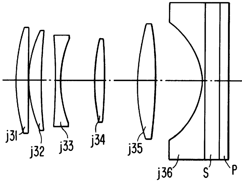
FIG. 6 PRIOR ART
