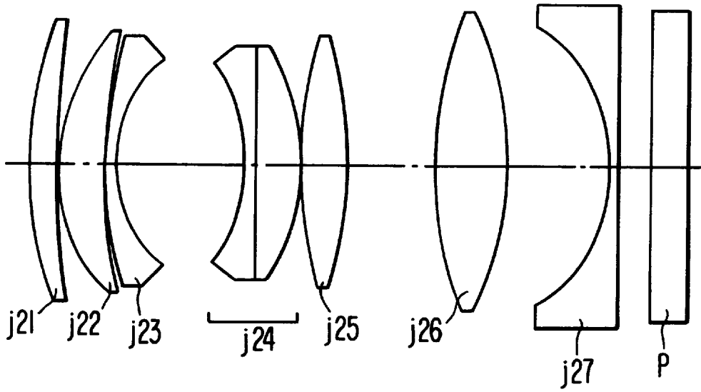
FIG. 5 PRIOR ART
