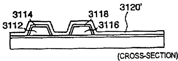
(f) SECOND METAL FILM (SILVER ALLOY) DEPOSITION
