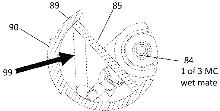
Fig. 5 B Section A-A Bottom view fluid flow path
