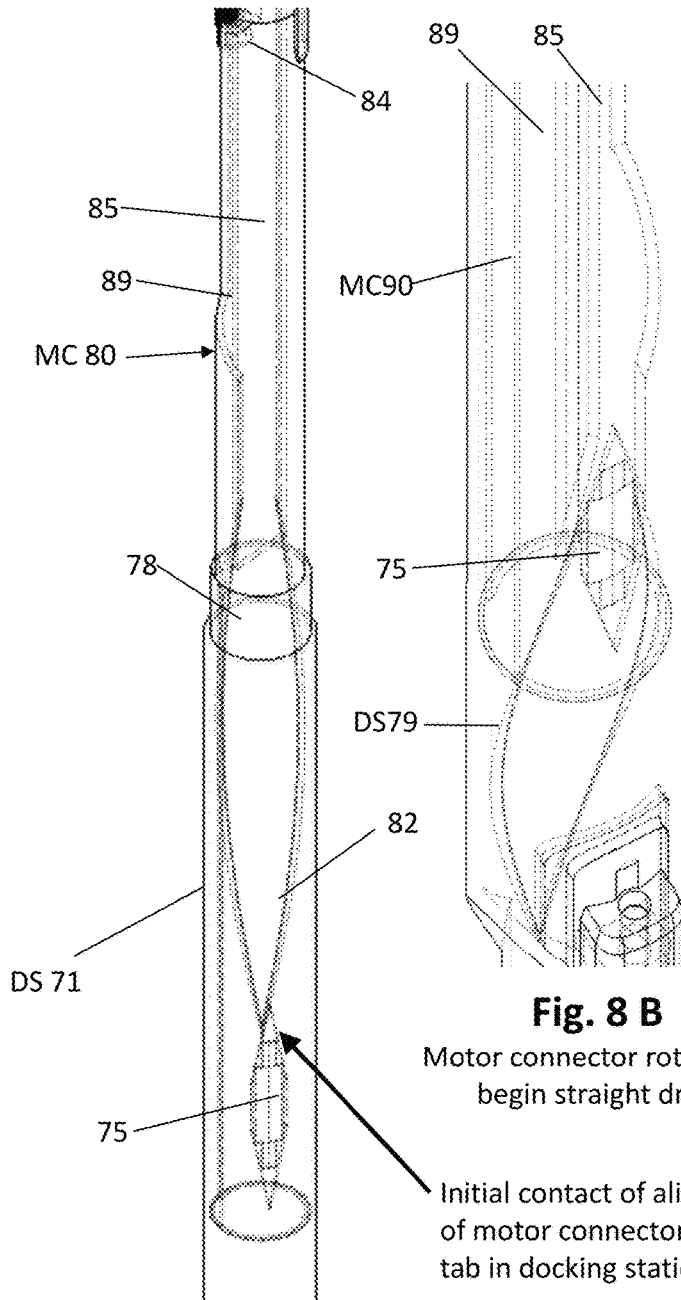
Fig. 8 A Motor connector rotation Spear function
