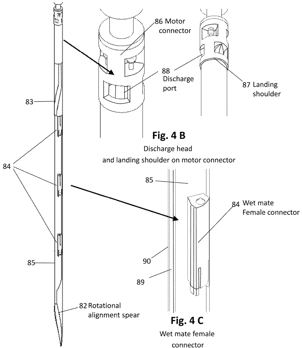
Fig. 4 A Discharge head and wet mate connector
