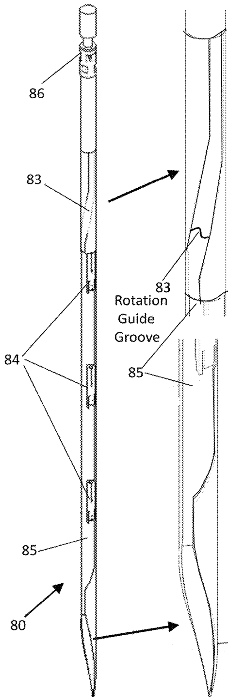
Fig. 3 A ESP/Motor connector alignment features
