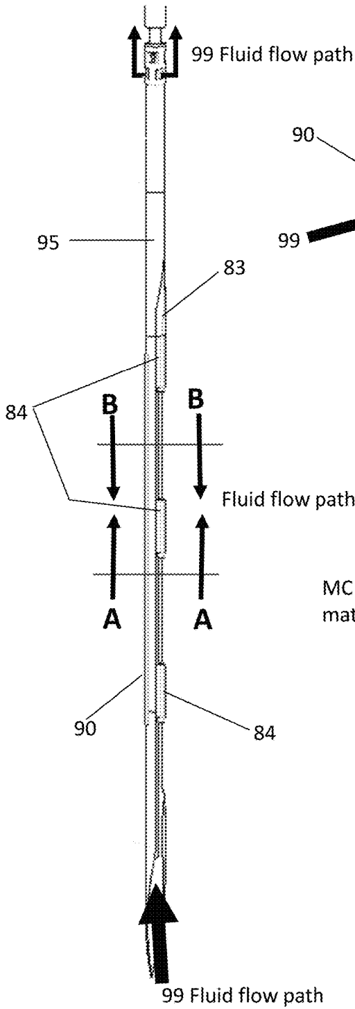
Fig. 5 A Fluid flow path through motor connector
