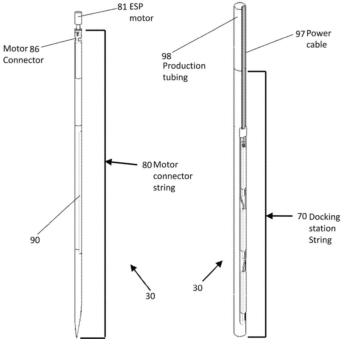
Fig. 1 A ESP/motor connector string 80
