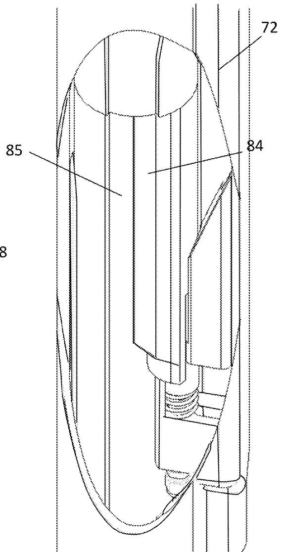
Fig. 11 B Final mate of wet mate connectors with shuttle body moving down to allow shuttle pin to insert in female connector
