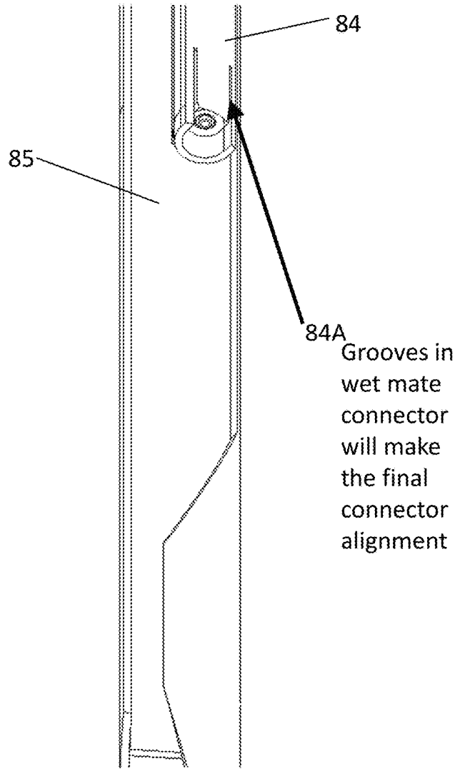
Fig. 10 B Bottom view of female wet mate connector
