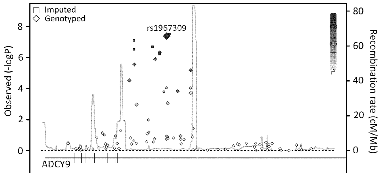
B. SNPs in the ADCY9 region
