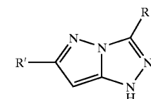
Pyrazolo[5,1-c]-1,2,4-triazole
