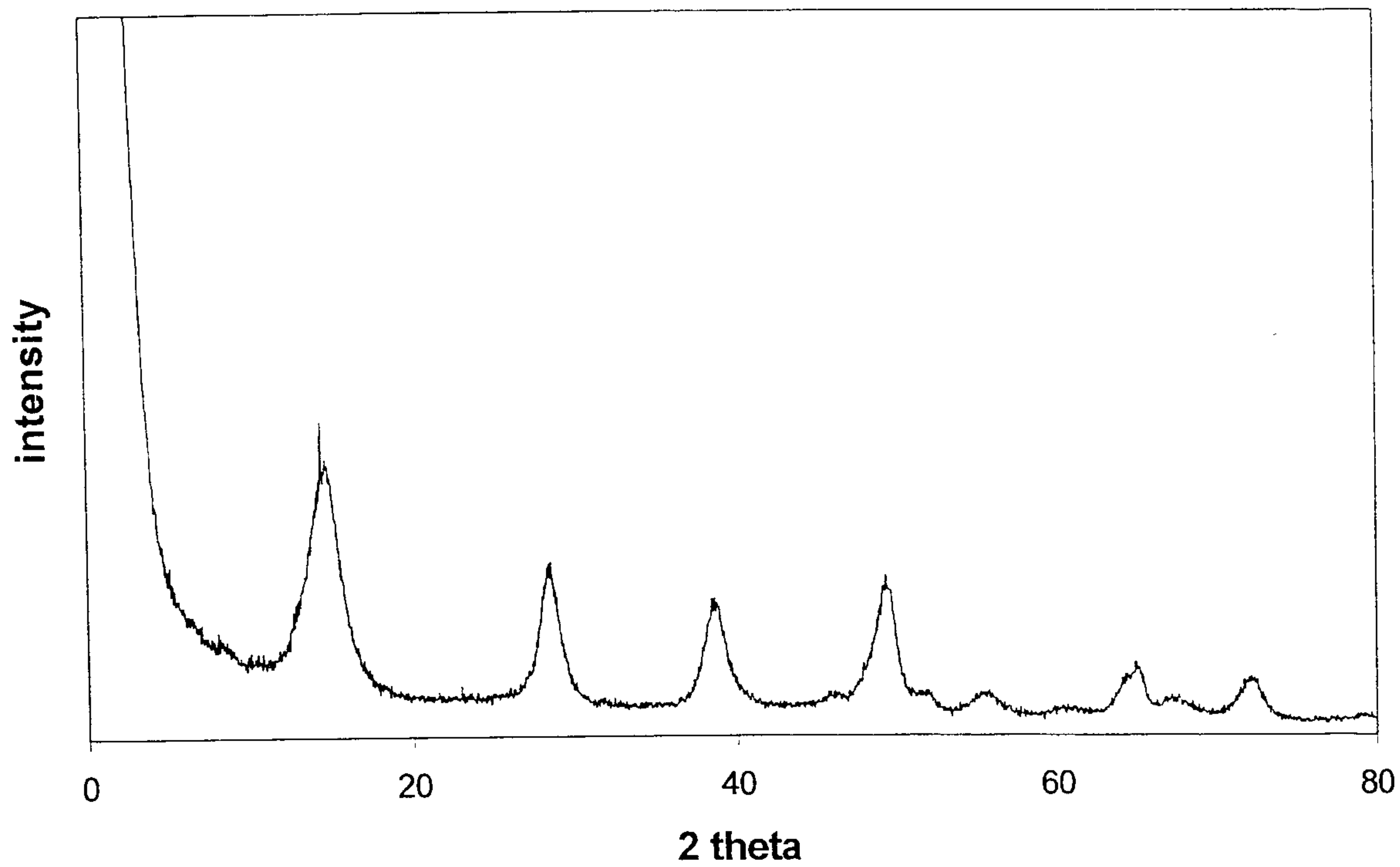
Figure 3 QCB prepared by hydrothermal treatment at pH=4
