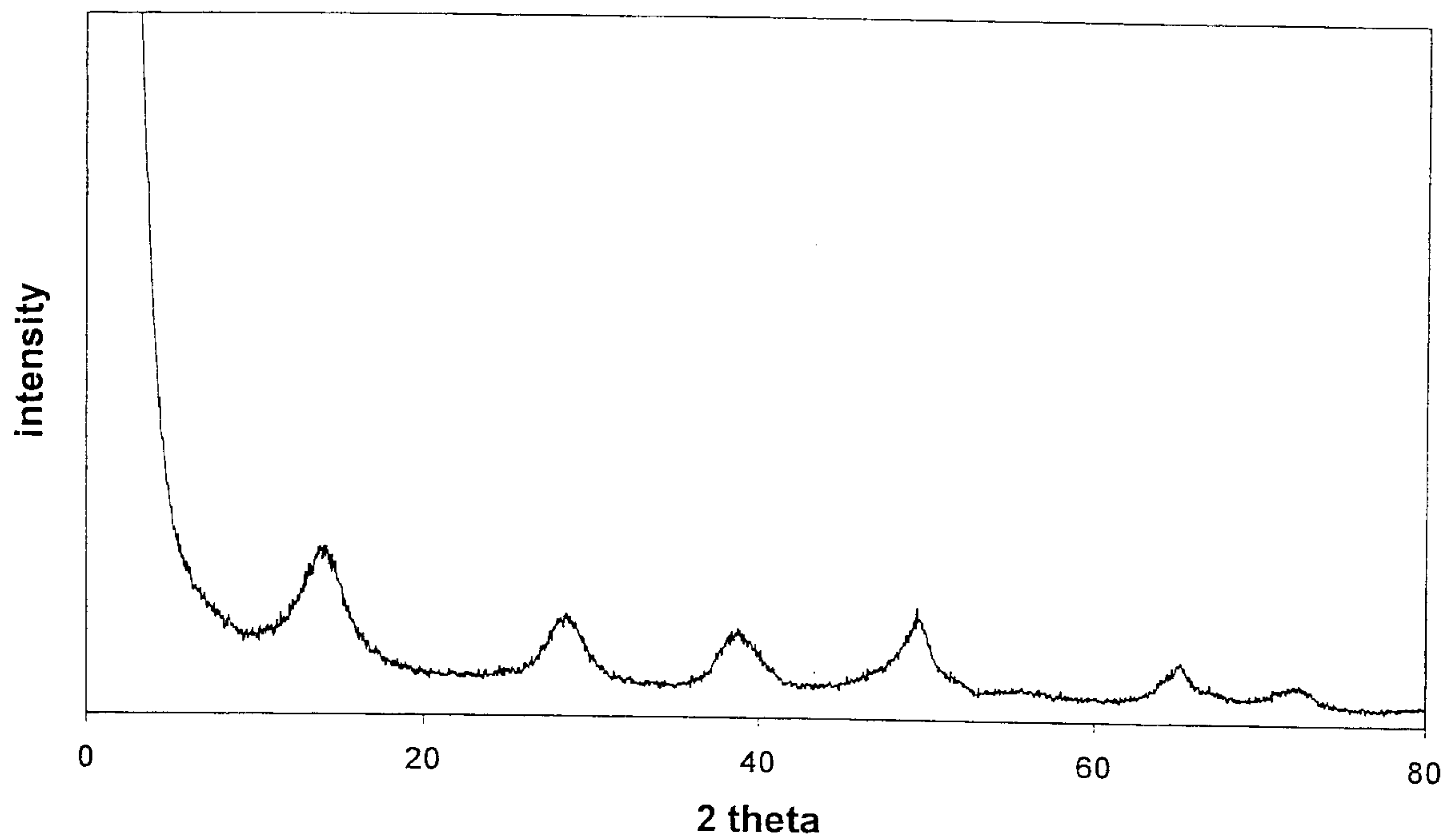
Figure 4 QCB prepared with Wachowski process
