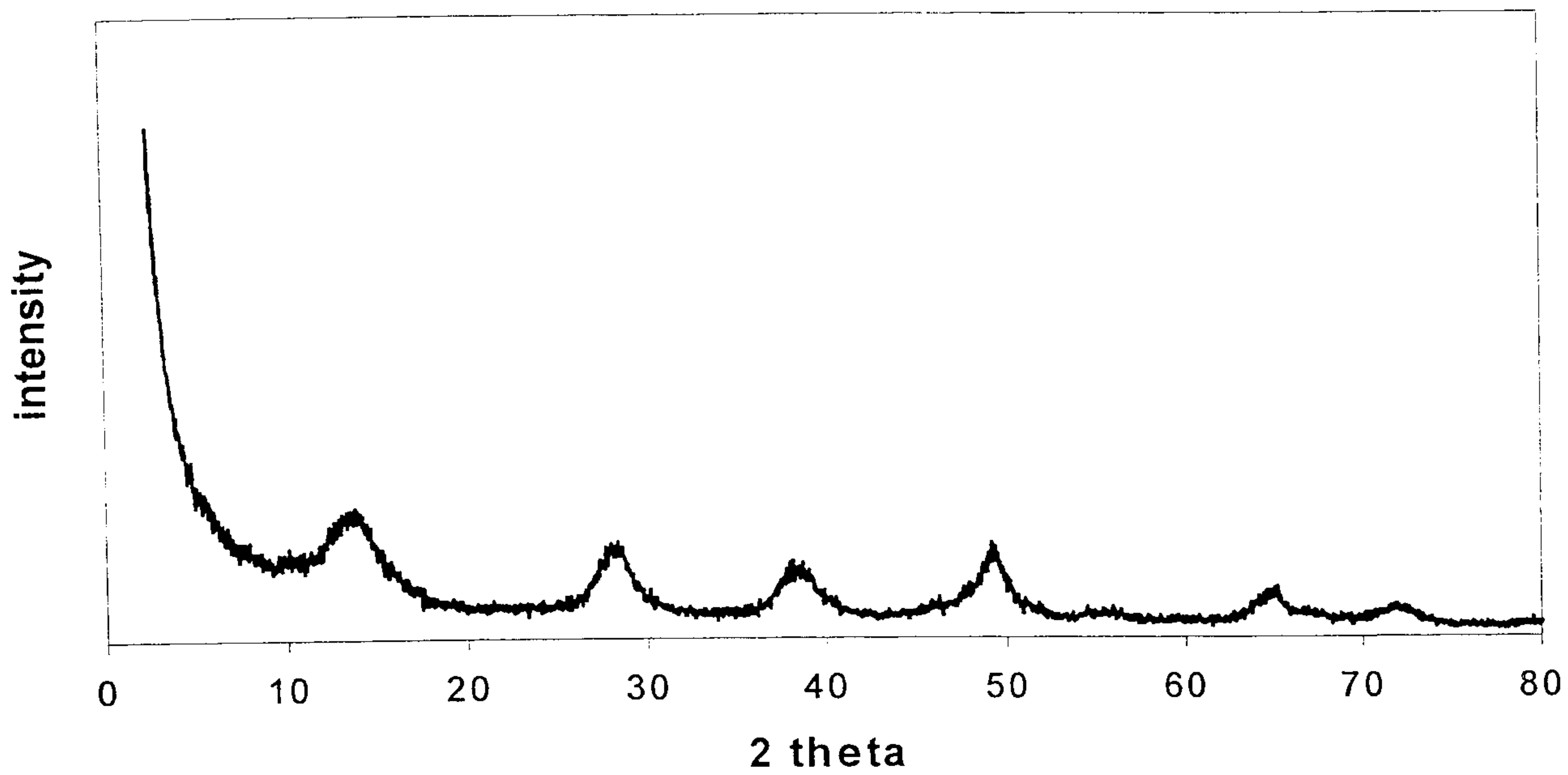
Figure 1. XRD of Catapal
