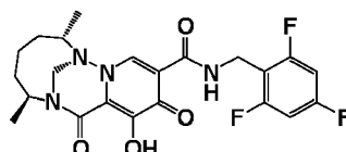
C23
