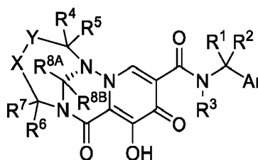
Formula Ib.
