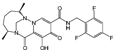
C8
