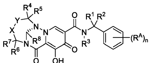
Formula IIb,
