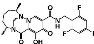
C22
