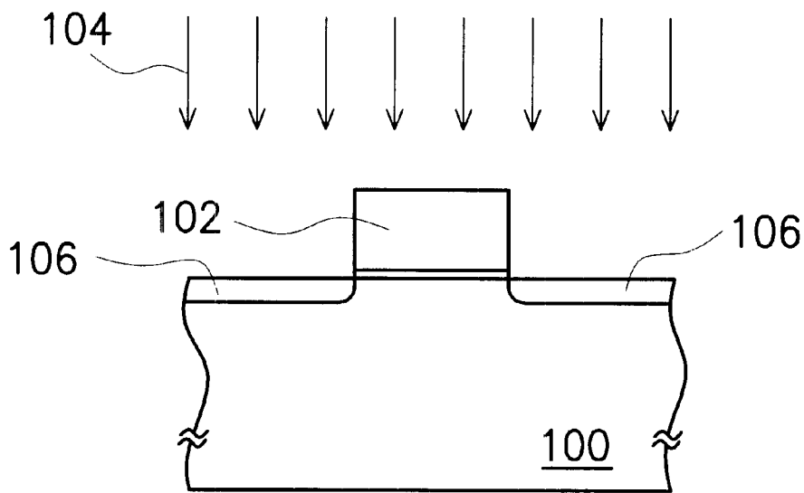
FIG. 1A(PRIOR ART)
