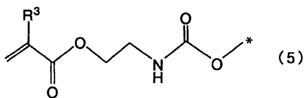
[Chemical Formula 5]
