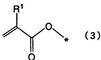
[Chemical Formula 3]
