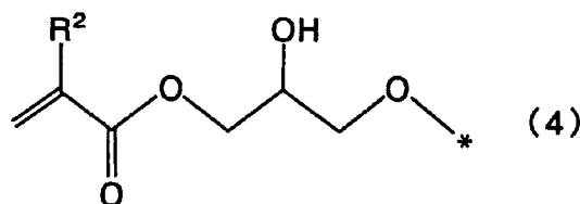
[Chemical Formula 10]
