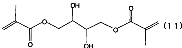
[Chemical Formula 18]
