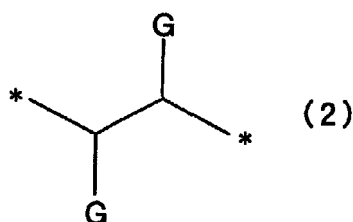
[Chemical Formula 12]
