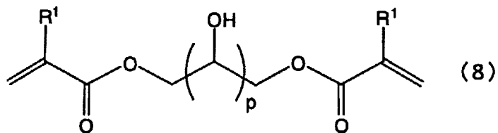
[Chemical Formula 8]
