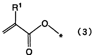
[Chemical Formula 4]
