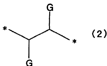
[Chemical Formula 2]
