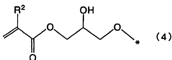
[Chemical Formula 4]
