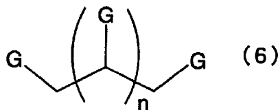
[Chemical Formula 6]
