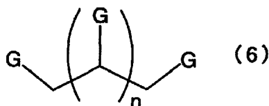
[Chemical Formula 13]
