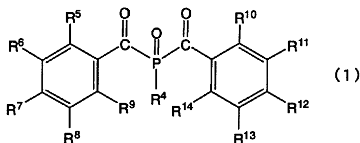
[Chemical Formula 1]
