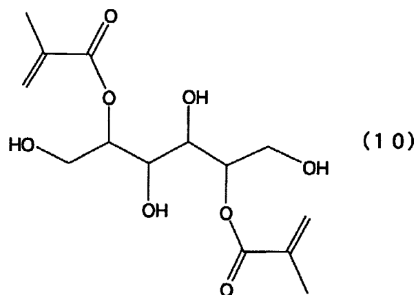
[Chemical Formula 16]
