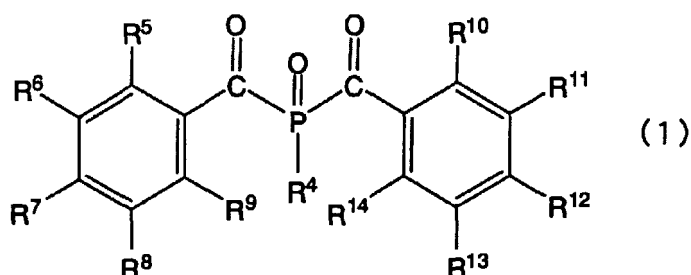
[Chemical Formula 1]
