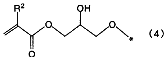
[Chemical Formula 4]
