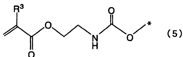
[Chemical Formula 5]
