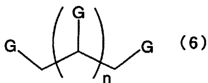
[Chemical Formula 6]
