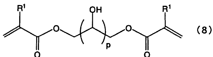
[Chemical Formula 17]
