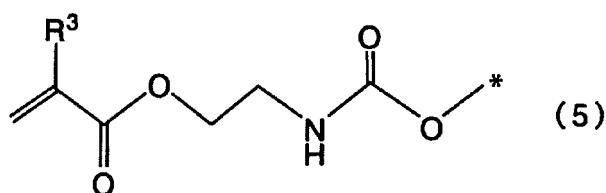
[Chemical Formula 11]
