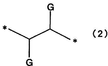
[Chemical Formula 2]
