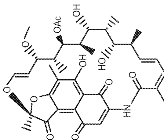
rifamycin S
