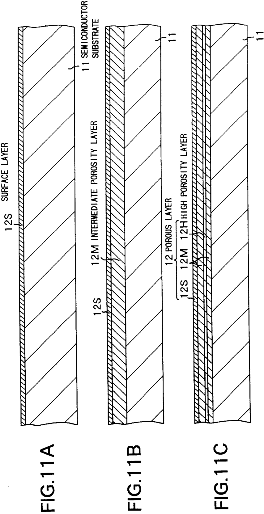
PROCESS DIAGRAM(FIRST)
