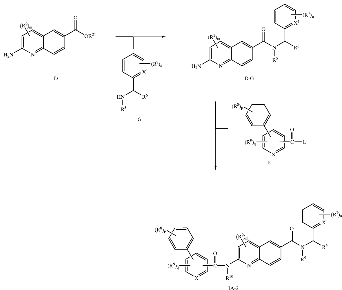
Scheme Ib
