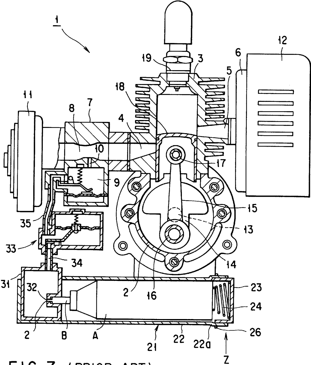
FIG. 7 (PRIOR ART)
