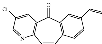
3-chloro-7-vinyl-5H-benzo[4,5]cyclohepta[1,2-b]pyridin-5-one (Compound 326)
