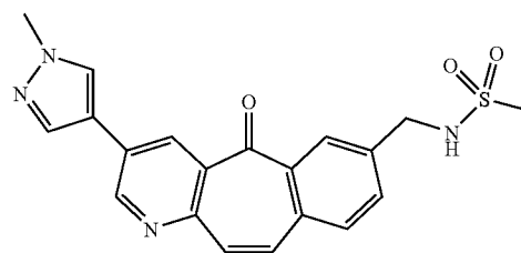
N-[[3-(1-methyl-1H-pyrazol-4-yl)-5-oxo-5H-benzo[4,5]cyclohepta[1,2-b]pyridin-7-yl]methyl]methanesulfonamide
