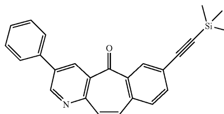
3-phenyl-7-[(trimethylsilyl)ethynyl]-5H-benzo[4,5]cyclohepta[1,2-b]pyridine-5-one
