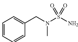
N-benzyl-N-methylsulfamide
