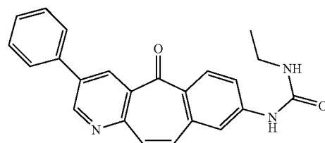
N-ethyl-N'-(5-oxo-3-phenyl-5H-benzo[4,5]cyclohepta[1,2-b]pyridin-8-yl)urea
