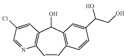
3-chloro-7-(1,2-dihydroxyethyl)-5H-benzo[4,5]cyclohepta[1,2-b]pyridin-5-one (Compound 339)
