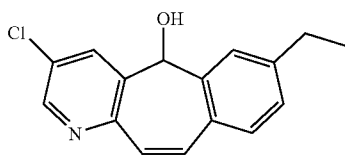
3-chloro-7-ethyl-5H-benzo[4,5]cyclohepta[1,2-b]pyridin-5-ol (Compound 338)
