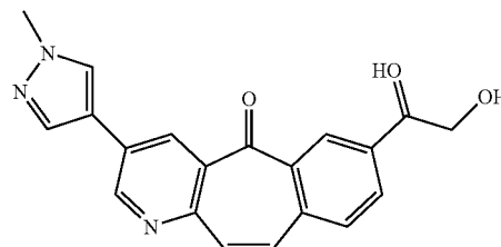
7-(1,2-dihydroxyethyl)-3-(1-methyl-1H-pyrazol-4-yl)-5H-benzo[4,5]cyclohepta[1,2-b]pyridin-5-one (Compound 340)
