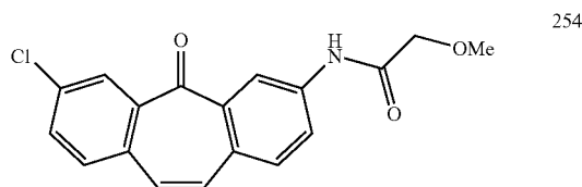
N-(3-chloro-5-oxo-5H-benzo[4,5]cyclohepta[1,2-b]pyridin-7-yl)-2-methoxyacetamide
