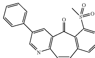
6-(methylsulfonyl)-3-phenyl-5H-benzo[4,5]cyclohepta[1,2-b]pyridin-5-one
