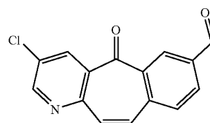
3-chloro-5-oxo-5H-benzo[4,5]cyclohepta[1,2-b]pyridine-7-carbaldehyde (Compound 341)
