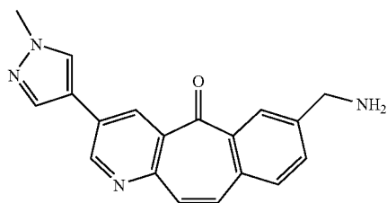
7-(aminomethyl)-3-(1-methyl-1H-pyrazol-4-yl)-5H-benzo[4,5]cyclohepta[1,2-b]pyridin-5-one
