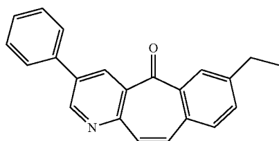
7-ethyl-3-phenyl-5H-benzo[4,5]cyclohepta[1,2-b]pyridin-5-one
