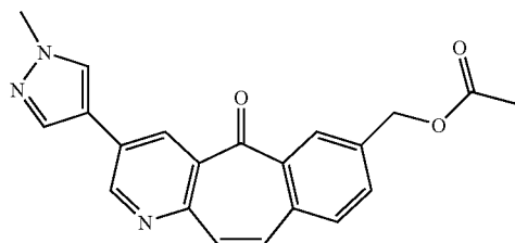
[3-(1-methyl-1H-pyrazol-4-yl)-5-oxo-5H-benzo[4,5] cyclohepta[1,2-b]pyridin-7-yl]methyl acetate (Com- pound 316)
