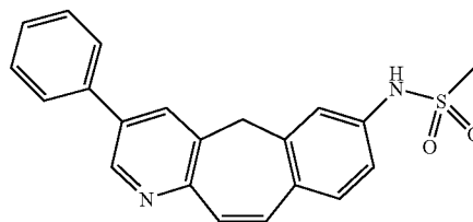
N-(3-phenyl-5H-benzo[4,5]cyclohepta[1,2-b]pyridin-7-yl)methanesulfonamide
