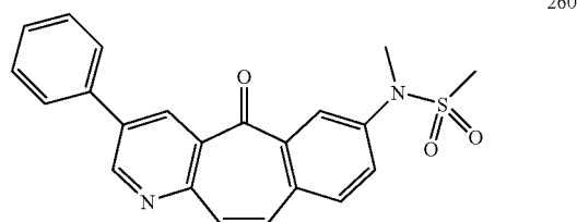
N-methyl-N-(5-oxo-3-phenyl-5H-benzo[4,5]cyclohepta[1,2-b]pyridin-7-yl)methanesulfonamide
