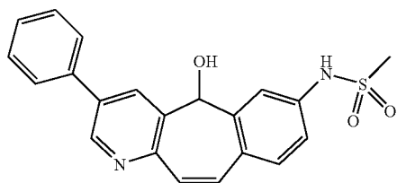
N-(5-hydroxy-3-phenyl-5H-benzo[4,5]cyclohepta[1,2-b]pyridin-7-yl)methanesulfonamide
