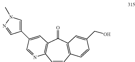
7-(hydroxymethyl)-3-(1-methyl-1H-pyrazol-4-yl)- 5H-benzo[4,5]cyclohepta[1,2-b]pyridin-5-one
