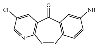
7-amino-3-chloro-5H-benzo[4,5]cyclohepta[1,2-b]pyridin-5-one
