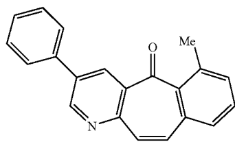
6-methyl-3-phenyl-5H-benzo[4,5]cyclohepta[1,2-b]pyridine-5-one
