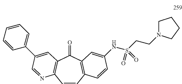
N-(5-oxo-3-phenyl-5H-benzo[4,5]cyclohepta[1,2-b]pyridin-7-yl)-2-pyrrolidin-1-ylethanesulfonamide
