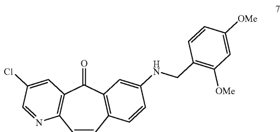
3-chloro-7-[(2,4-dimethoxybenzyl)amino]-5H-benzo[4,5]cyclohepta[1,2-b]pyridin-5-one
