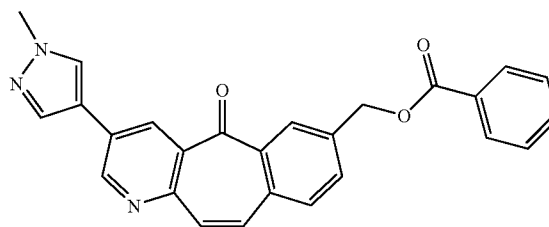
[3-(1-methyl-1H-pyrazol-4-yl)-5-oxo-5H-benzo[4,5] cyclohepta[1,2-b]pyridin-7-yl]methyl benzoate (Compound 317)
