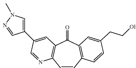
7-(2-hydroxyethyl)-3-(1-methyl-1H-pyrazol-4-yl)-5H-benzo[4,5]cyclohepta[1,2-b]pyridin-5-one (Compound 336)
