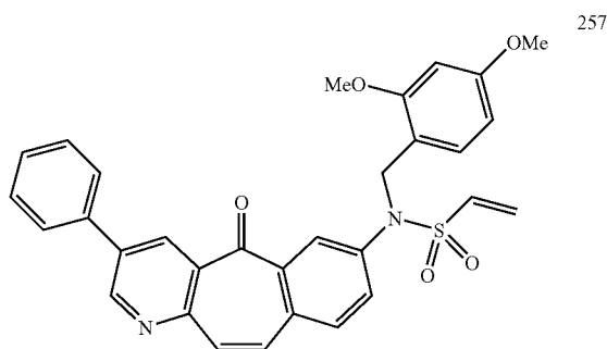
N-(2,4-dimethoxybenzyl)-N-(5-oxo-3-phenyl-5H-benzo[4,5]cyclohepta[1,2-b]pyridin-7-yl)ethanesulfonamide
