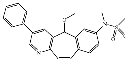
N-(5-methoxy-3-phenyl-5H-benzo[4,5]cyclohepta[1,2-b]pyridin-7-yl)-N-methylmethanesulfonamide
