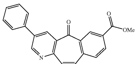
Methyl 5-oxo-3-phenyl-5H-benzo[4,5]cyclohepta[1,2-b]pyridine-7-carboxylate
