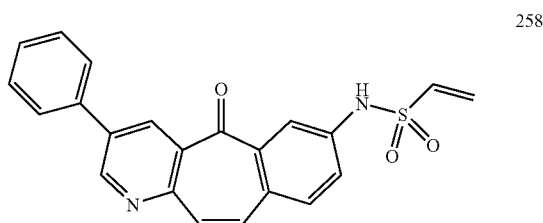
N-(5-oxo-3-phenyl-5H-benzo[4,5]cyclohepta[1,2-b]pyridin-7-yl)ethanesulfonamide
