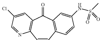
N-(3-chloro-5-oxo-5H-benzo[4,5]cyclohepta[1,2-b]pyridin-7-yl)methanesulfonamide
