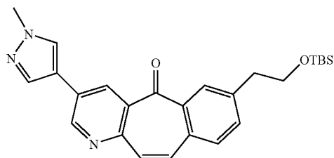
7-(2-[[tert-butyl(dimethyl)silyl]oxy]ethyl)-3-(1-methyl-1H-pyrazol-4-yl)-5H-benzo[4,5]cyclohepta[1,2-b]pyridin-5-one (Compound 335)
