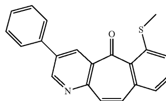
6-(methylthio)-3-phenyl-5H-benzo[4,5]cyclohepta[1,2-b]pyridin-5-one
