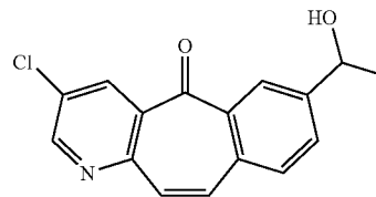
3-chloro-7-(1-hydroxyethyl)-5H-benzo[4,5]cyclohepta[1,2-b]pyridin-5-one (Compound 337)
