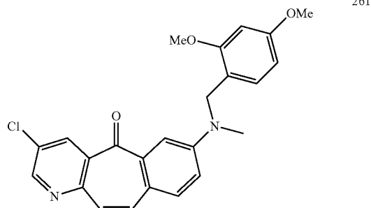
3-chloro-7-[(2,4-dimethoxybenzyl)(methyl)amino]-5H-benzo[4,5]cyclohepta[1,2-b]pyridin-5-one
