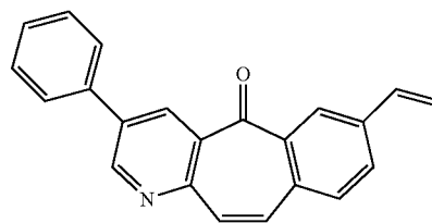
3-phenyl-7-vinyl-5H-benzo[4,5]cyclohepta[1,2-b]pyridine-5-one
