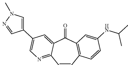
7-(isopropylamino)-3-(1-methyl-1H-pyrazol-4-yl)-5H-benzo[4,5]cyclohepta[1,2-b]pyridin-5-one
