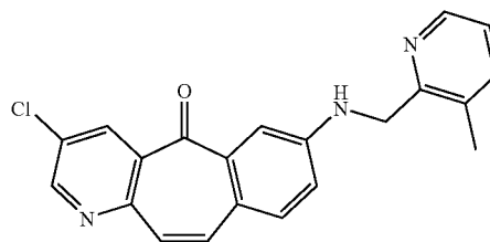
3-chloro-7-[(3-methylpyridin-2-yl)methyl]amino)-5H-benzo[4,5]cyclohepta[1,2-b]pyridin-5-one (Compound 56)
