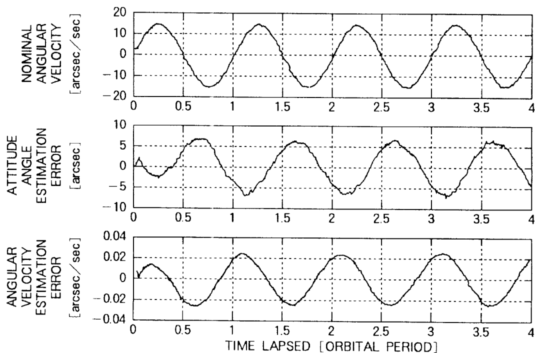
(b) CASE OF TIME-DEPENDENT VARIABLE NOMINAL ANGULAR VELOCITY
