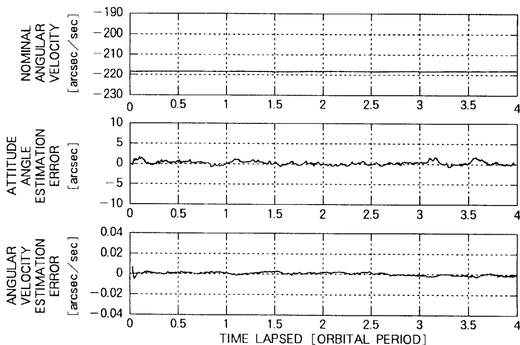
(a) CASE OF CONSTANT NOMINAL ANGULAR VELOCITY
