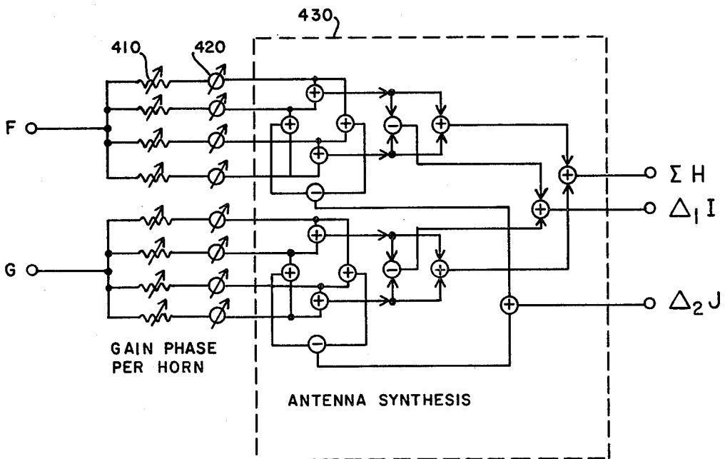
Fig. 8 ANTENNA SYNTHESIS
