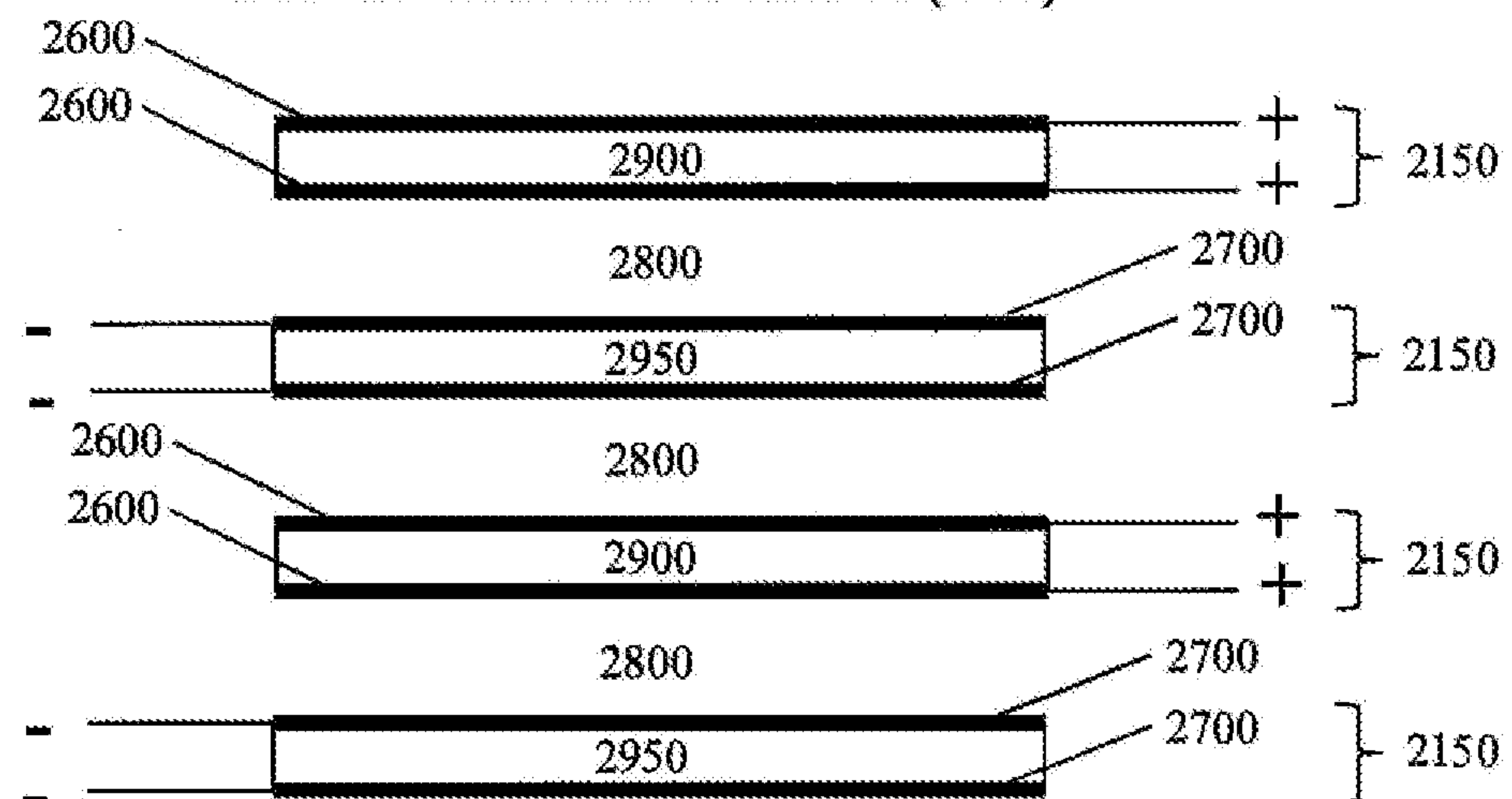
MULTI-ELECTRODE ARRAY (2100)
