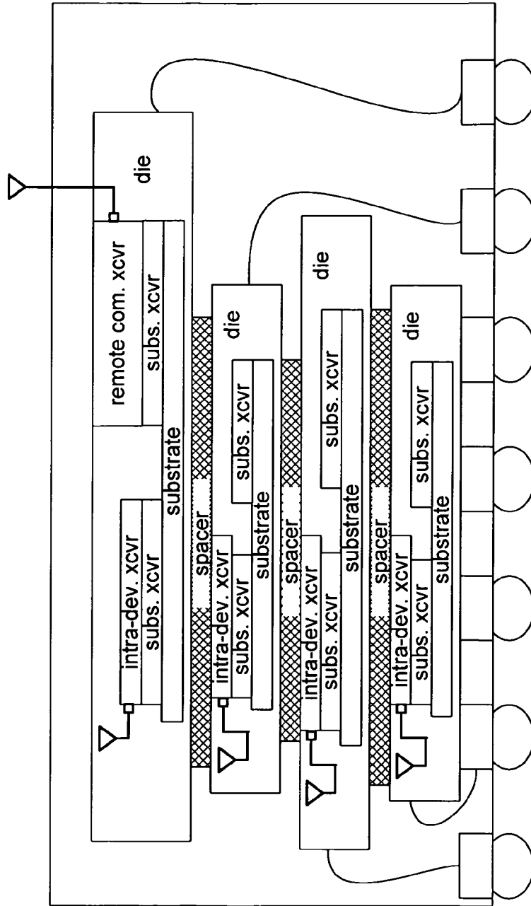
multi-chip module 330
