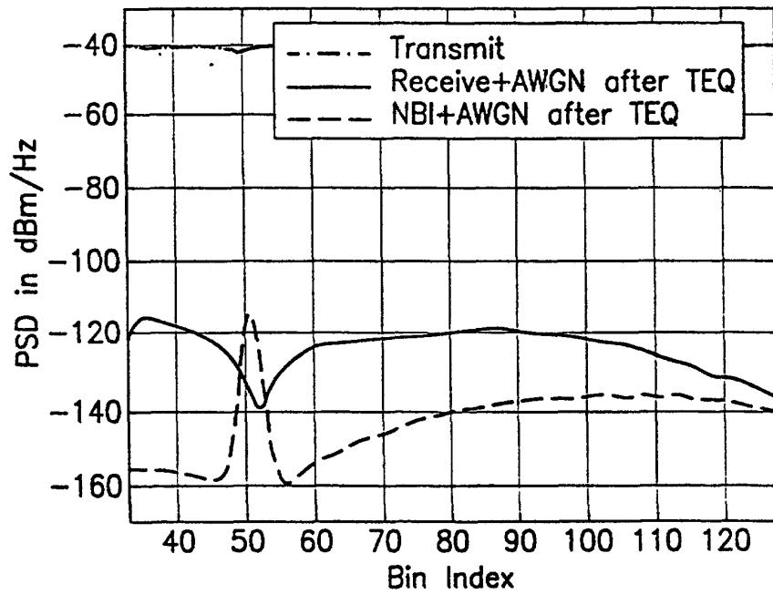
Long Loop With NBI Signal And Noise PSD'S After TEQ
