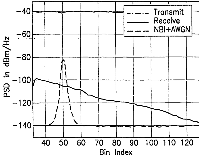
Long Loop With NBI Signal And Noise PSD'S Before TEQ
