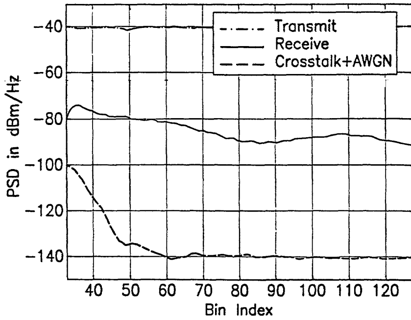
Medium Loop With Crosstalk Signal And Noise PSD'S Before TEQ
