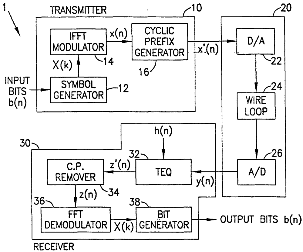
Fig. 14 (Prior Art)
