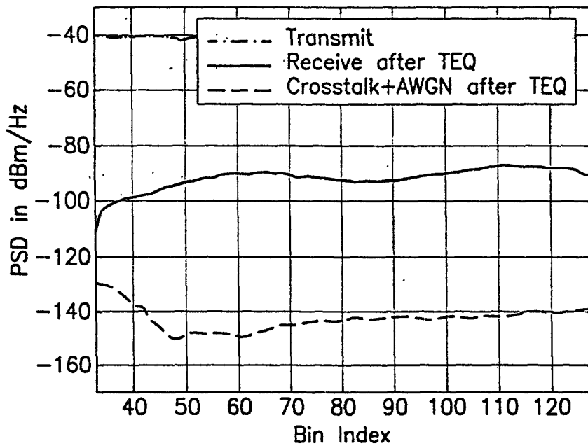
Medium Loop With Crosstalk Signal And Noise PSD'S After TEQ
