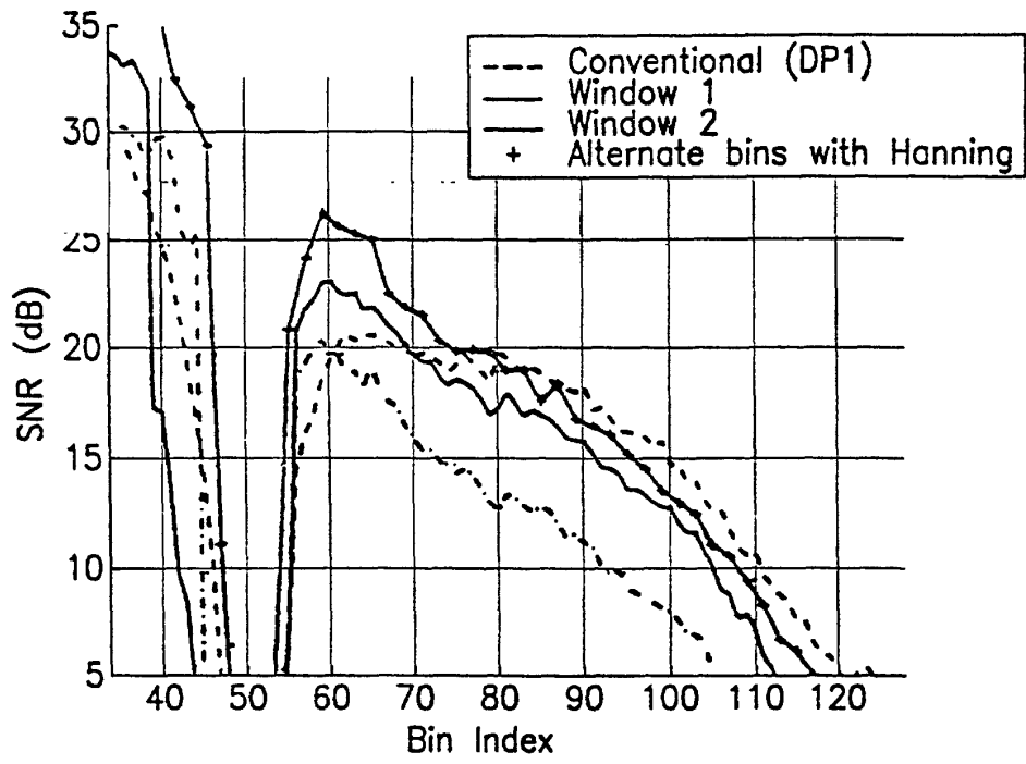
Long Loop With NBI Profile
