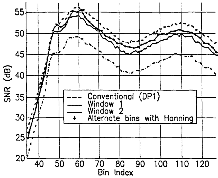
Medium Loop With Crosstalk SNR Profile
