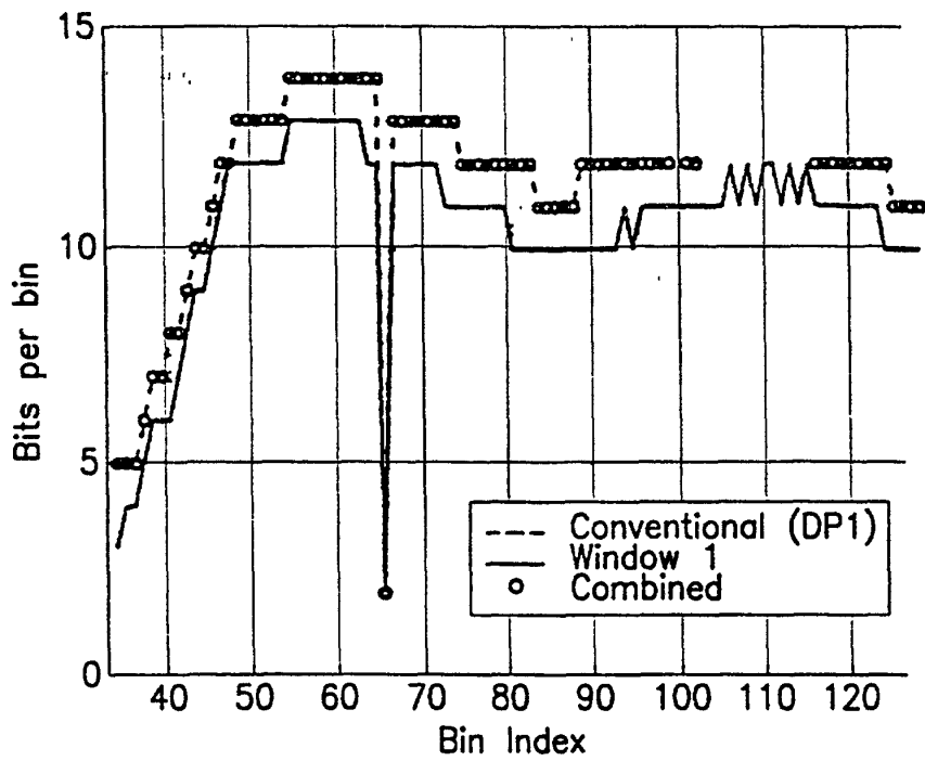
Medium Loop With Crosstalk Bit Allocation Profile
