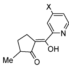
Compound 23a
