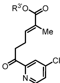
Compound 18
