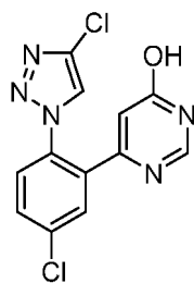
Compound 14
