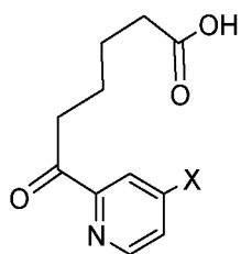
Compound 4
