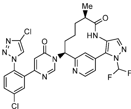
Compound (I).
