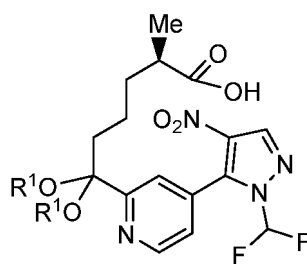
Compound 9
