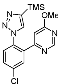
Compound 46;
