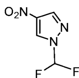
Compound 8
