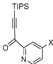
Compound 29
