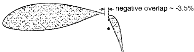
Fig. 2(b) airfoil SA-21 - large flap deflections, \delta_{\text{flap}} = +60\text{deg} , negative overlap, continuation of simple mechanical rotation around hinge point
