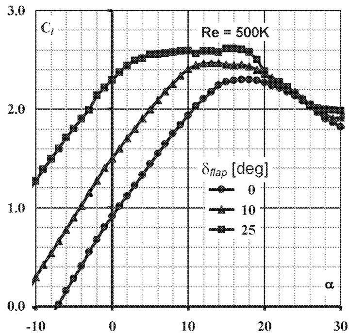
Fig. 17(a) conventional flap deflections
