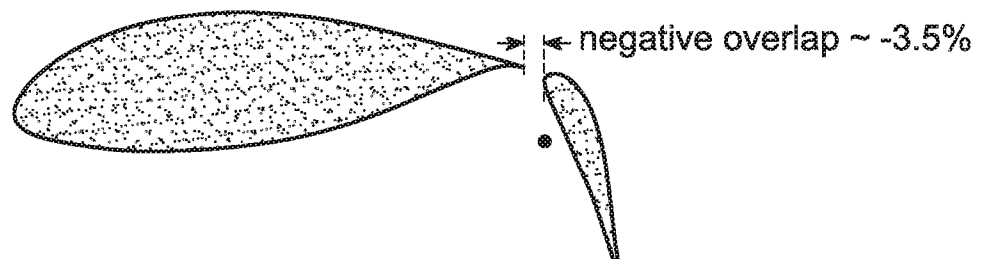
Fig. 2(b) airfoil SA-21 - large flap deflections, \delta_{\text{flap}} = +60\text{deg} , negative overlap, continuation of simple mechanical rotation around hinge point
