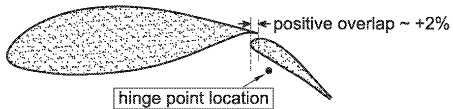
Fig. 2(a) airfoil SA-21 - conventional flap deflections, \delta_{\text{flap}} = +25\text{deg} , positive overlap
