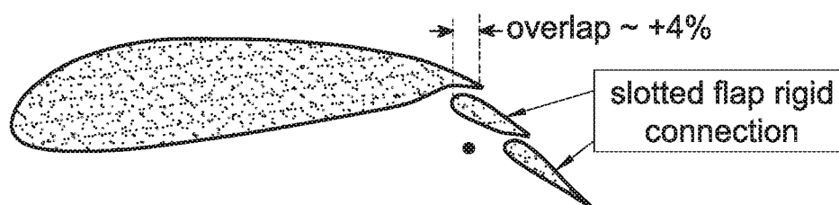
Fig. 7(b) maximum conventional flap deflection, \delta_{\text{flap}} = +25^\circ
