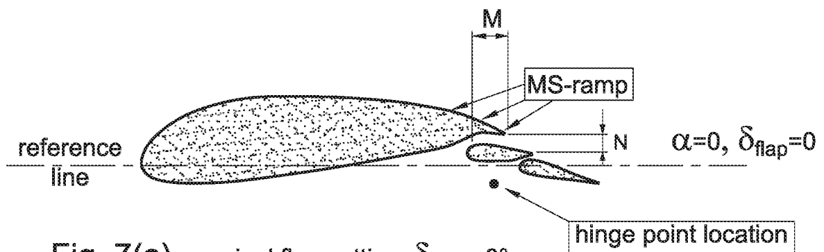
Fig. 7(a) nominal flap setting, \delta_{\text{flap}} = 0^\circ
