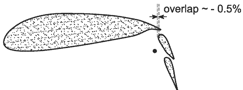
Fig. 7(c) deployed airbrake, \delta_{\text{flap}} = +60^\circ
