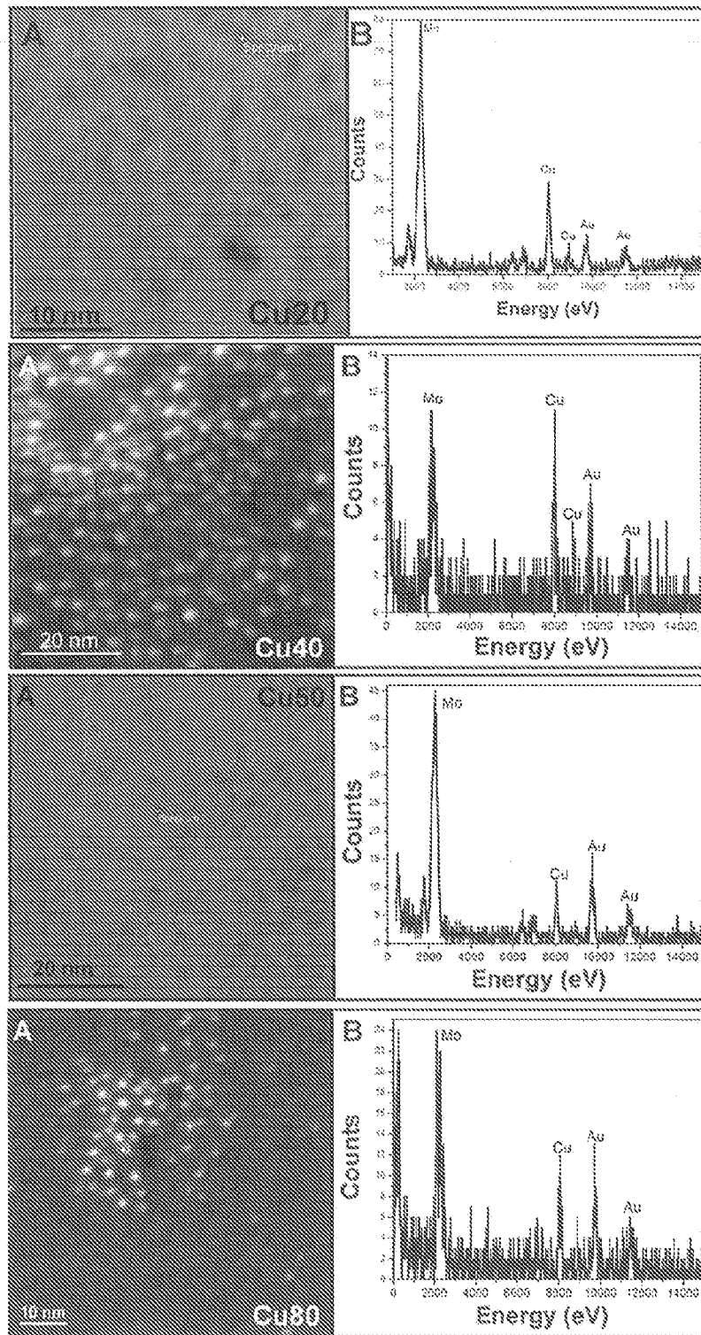
representative STEM (A) and corresponding EDS spectra (B) of Au x Cu y NPs (Cu 20 , Cu 40 , Cu 50 , and Cu 80 ) on molybdenum 400 mesh grids.
