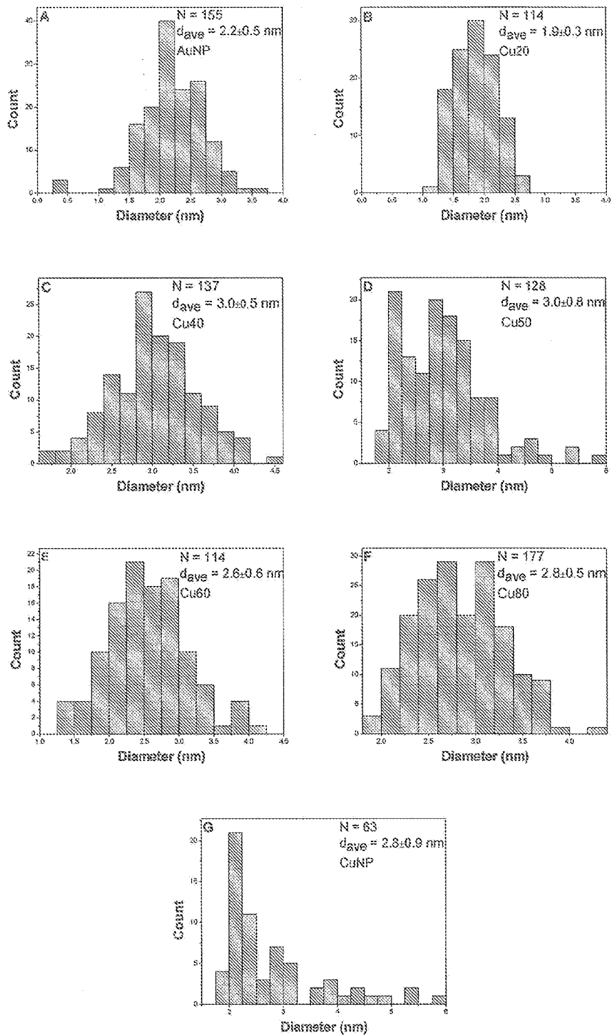
Histograms showing the diameter distribution of AuNP (A), Cu20 (B), Cu40 (C), Cu50 (D), Cu60 (E), Cu80(F), and CuNP (G).
